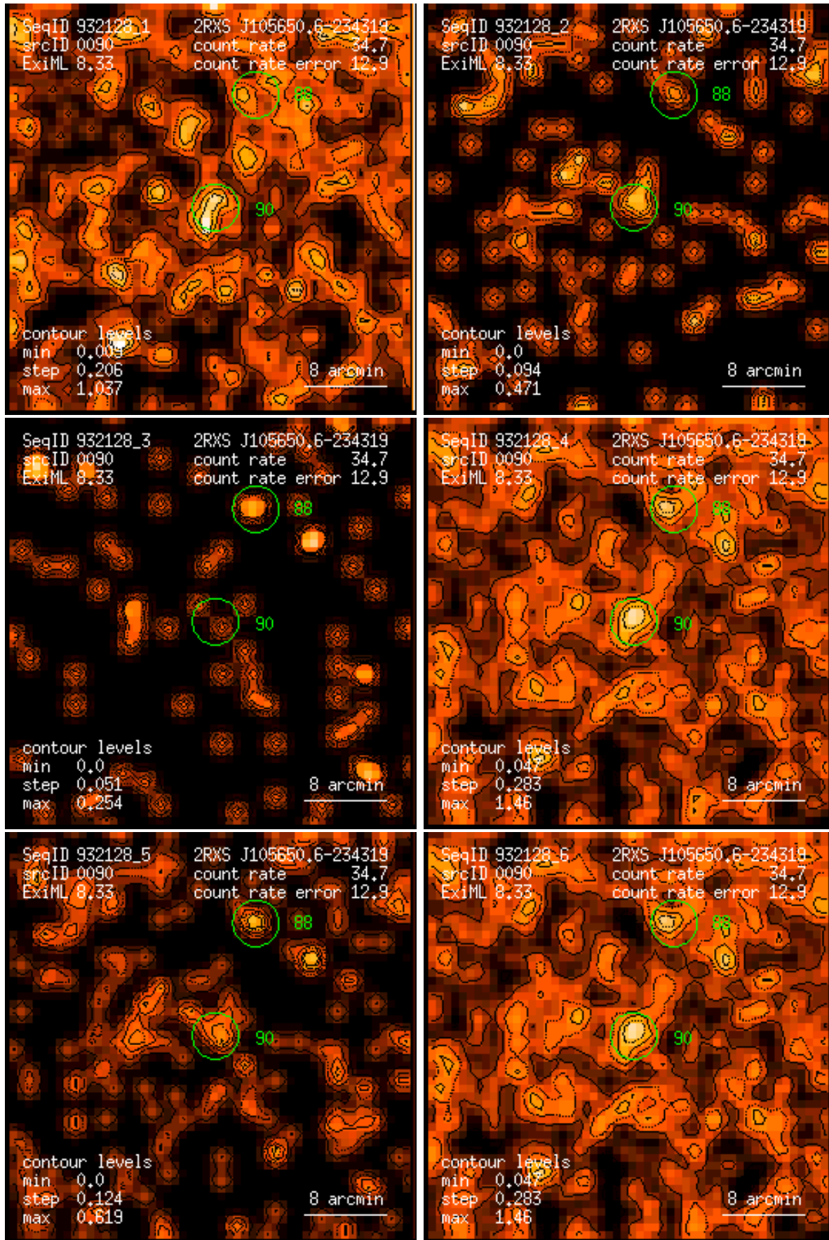
Figure 90: RASS 932128: detection 0090: band rate images, Gaussian filter: (1) PSPC channels 11 – 41, (2) 52 – 90, (3) 91 – 201, (4) 11 – 235, (5) 52 – 201, (6) 11 – 201. Broad band rates in counts/ks. Band rate contour levels in counts/ks/arcmin 2 .
