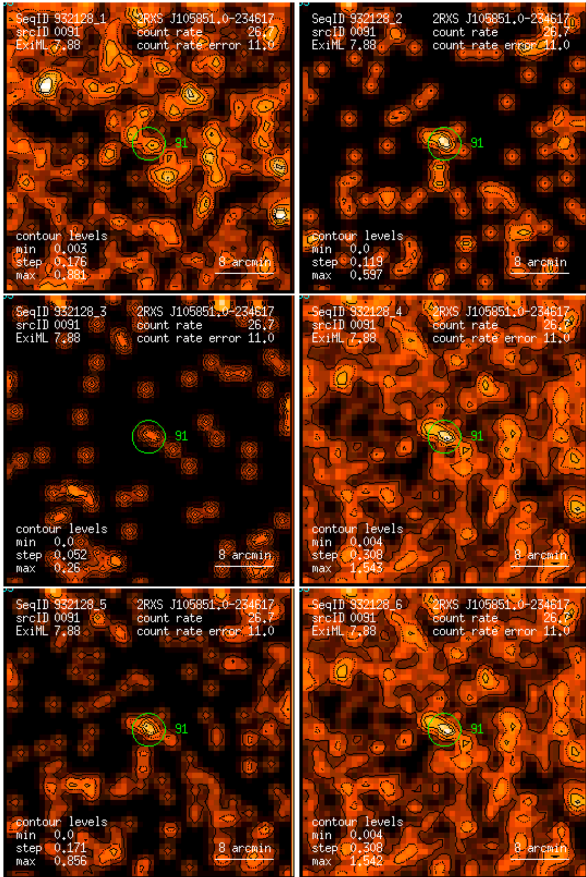
Figure 91: RASS 932128: detection 0091: band rate images, Gaussian filter: (1) PSPC channels 11 – 41, (2) 52 – 90, (3) 91 – 201, (4) 11 – 235, (5) 52 – 201, (6) 11 – 201. Broad band rates in counts/ks. Band rate contour levels in counts/ks/arcmin 2 .
