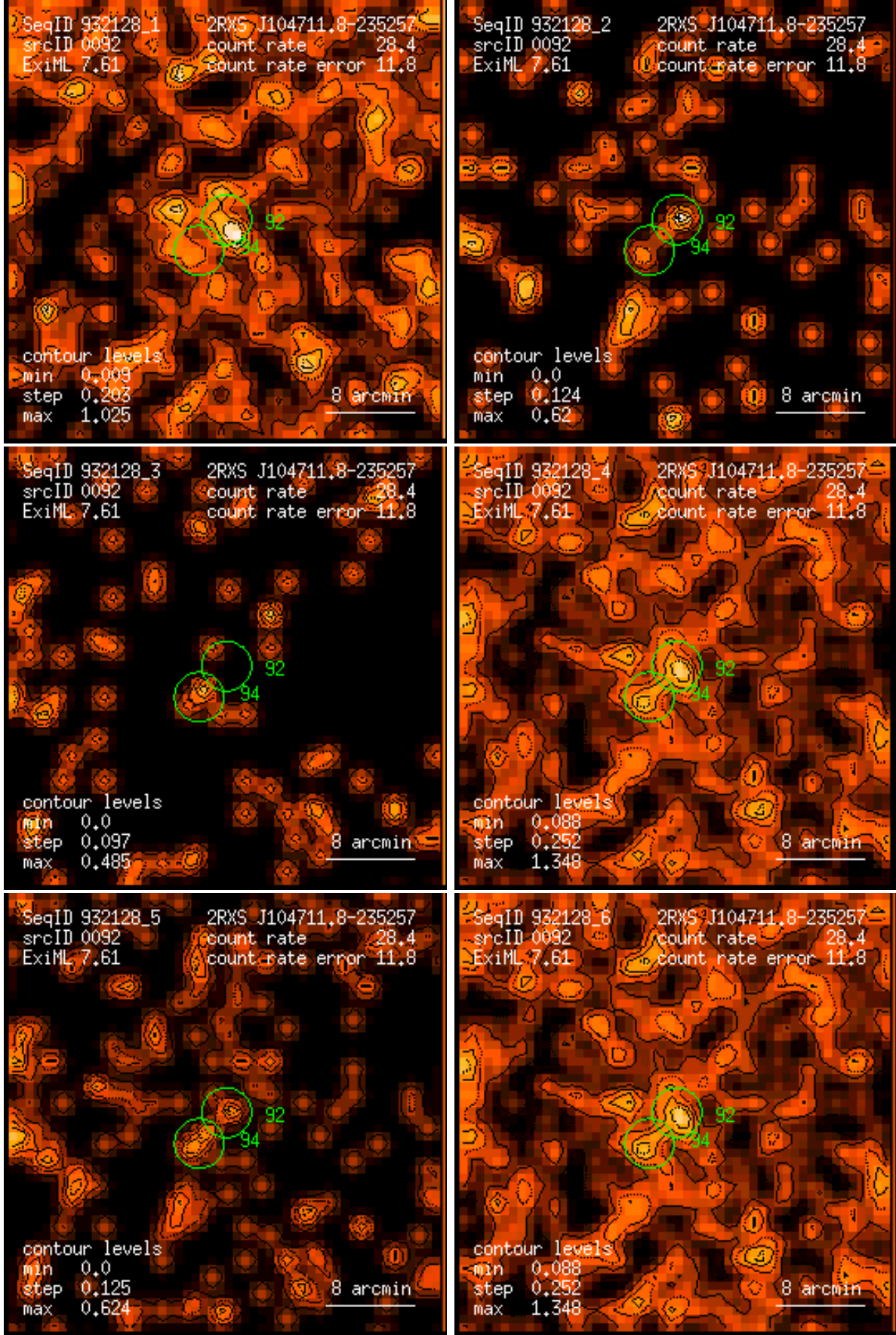
Figure 92: RASS 932128: detection 0092: band rate images, Gaussian filter: (1) PSPC channels 11 – 41, (2) 52 – 90, (3) 91 – 201, (4) 11 – 235, (5) 52 – 201, (6) 11 – 201. Broad band rates in counts/ks. Band rate contour levels in counts/ks/arcmin 2 .
