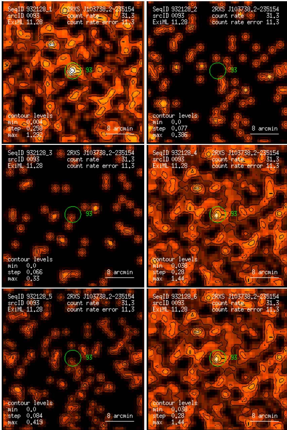
Figure 93: RASS 932128: detection 0093: band rate images, Gaussian filter: (1) PSPC channels 11 – 41, (2) 52 – 90, (3) 91 – 201, (4) 11 – 235, (5) 52 – 201, (6) 11 – 201. Broad band rates in counts/ks. Band rate contour levels in counts/ks/arcmin 2 .
