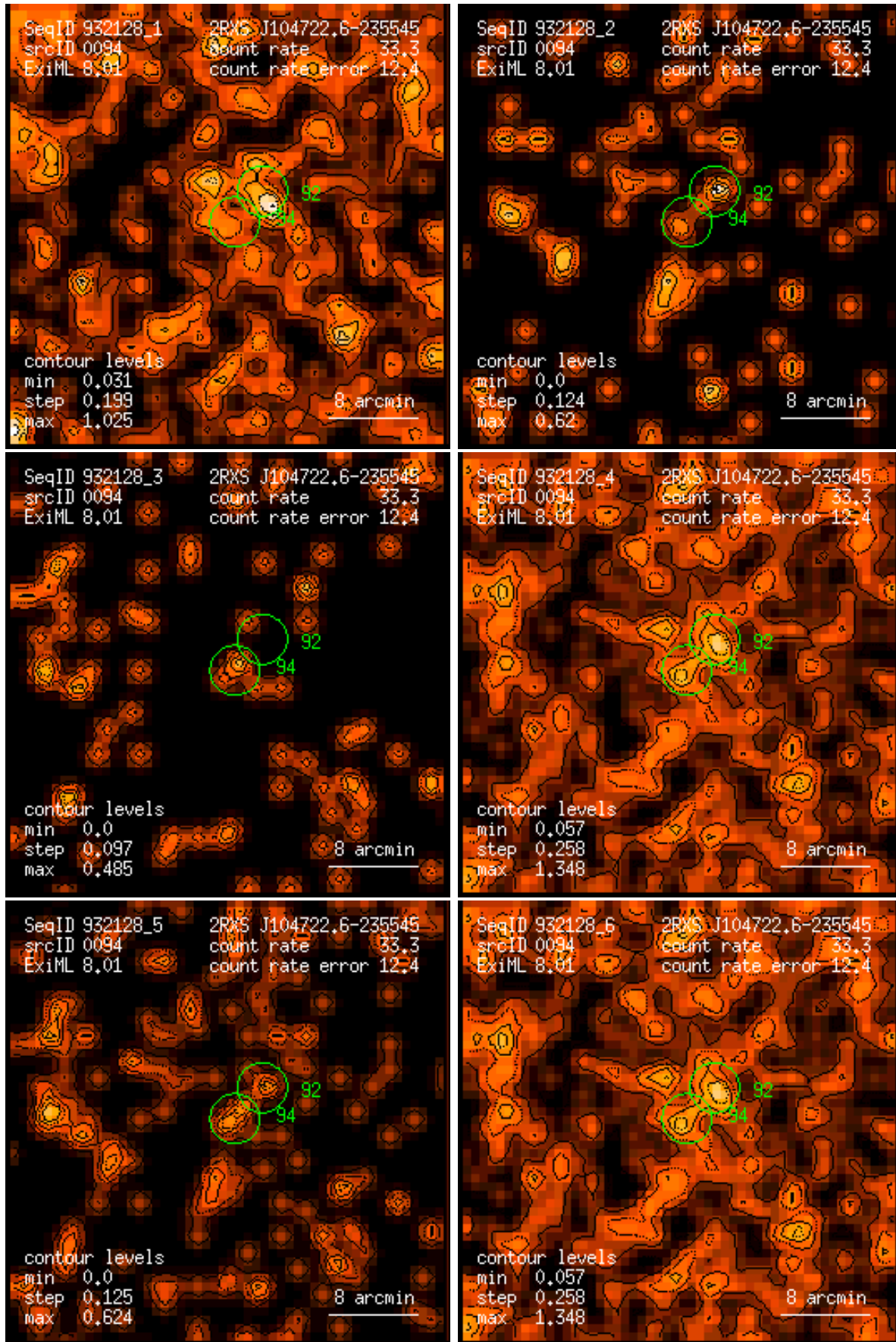
Figure 94: RASS 932128: detection 0094: band rate images, Gaussian filter: (1) PSPC channels 11 – 41, (2) 52 – 90, (3) 91 – 201, (4) 11 – 235, (5) 52 – 201, (6) 11 – 201. Broad band rates in counts/ks. Band rate contour levels in counts/ks/arcmin 2 .
