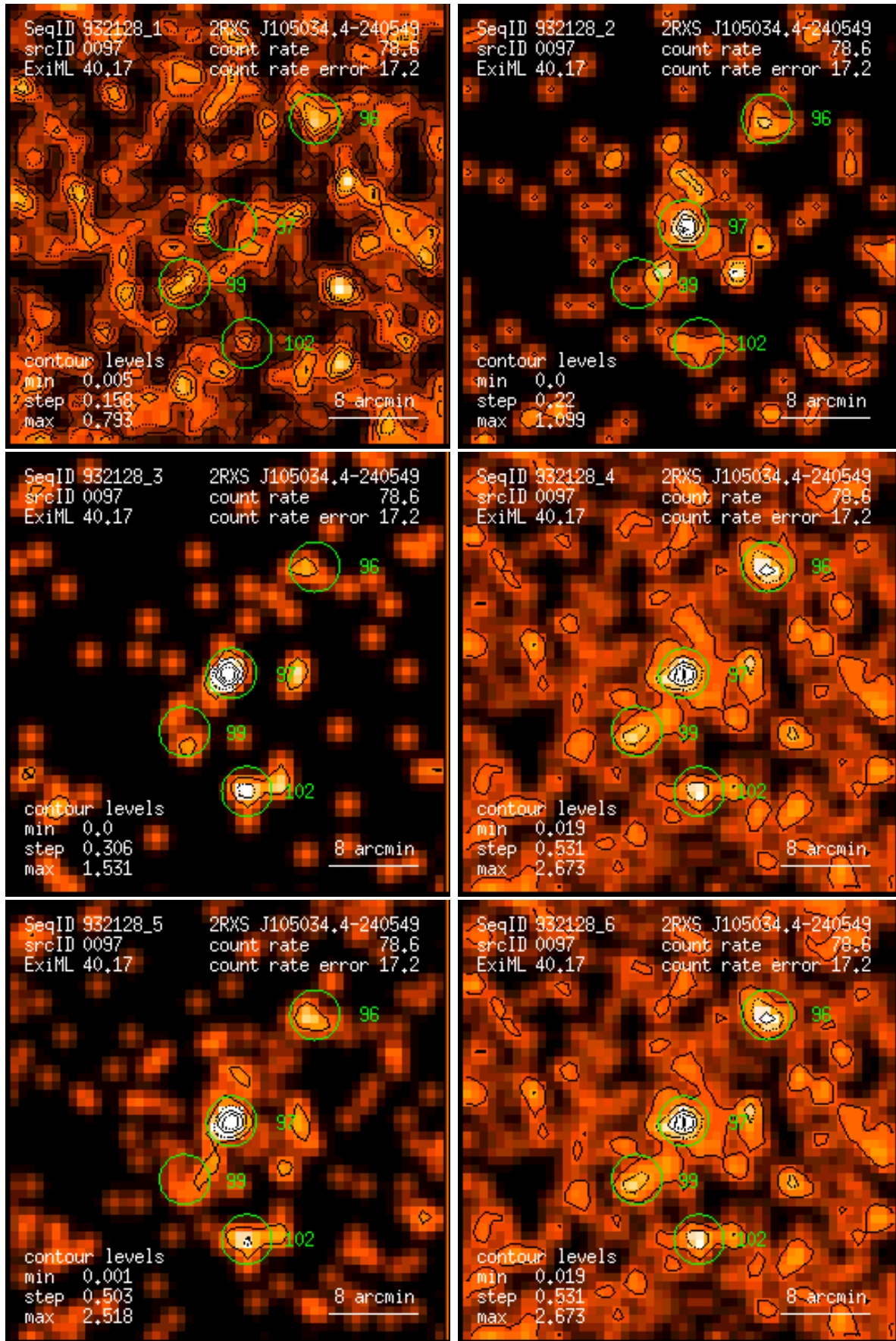
Figure 97: RASS 932128: detection 0097: band rate images, Gaussian filter: (1) PSPC channels 11 – 41, (2) 52 – 90, (3) 91 – 201, (4) 11 – 235, (5) 52 – 201, (6) 11 – 201. Broad band rates in counts/ks. Band rate contour levels in counts/ks/arcmin 2 .
