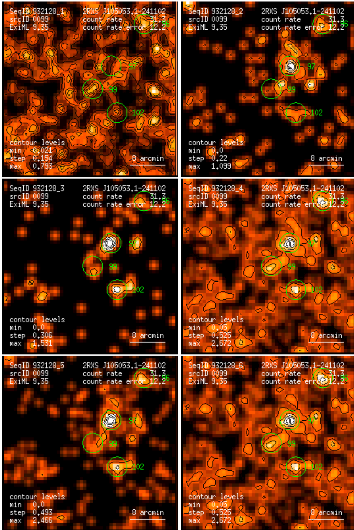
Figure 99: RASS 932128: detection 0099: band rate images, Gaussian filter: (1) PSPC channels 11 – 41, (2) 52 – 90, (3) 91 – 201, (4) 11 – 235, (5) 52 – 201, (6) 11 – 201. Broad band rates in counts/ks. Band rate contour levels in counts/ks/arcmin 2 .
