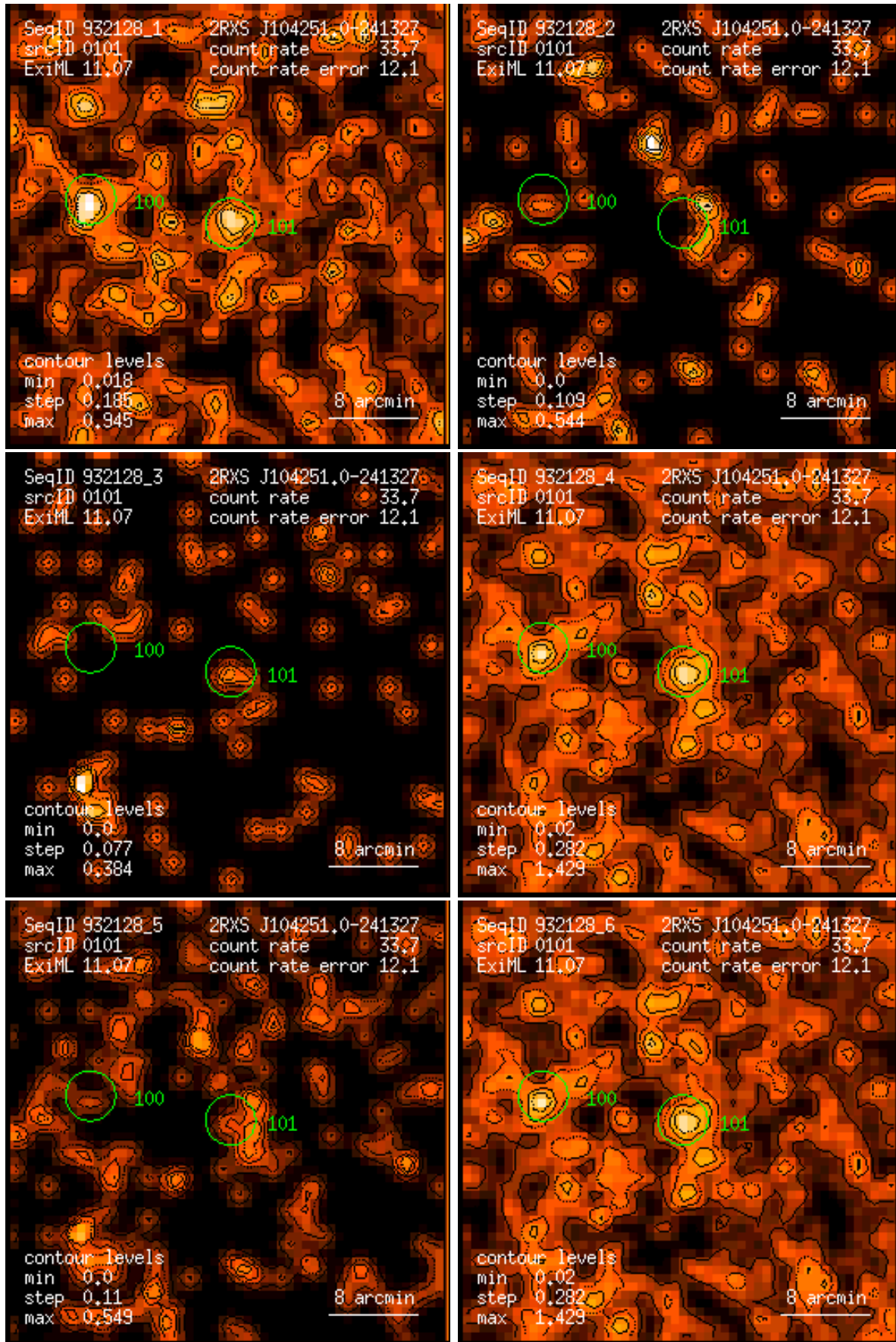
Figure 101: RASS 932128: detection 0101: band rate images, Gaussian filter: (1) PSPC channels 11 – 41, (2) 52 – 90, (3) 91 – 201, (4) 11 – 235, (5) 52 – 201, (6) 11 – 201. Broad band rates in counts/ks. Band rate contour levels in counts/ks/arcmin 2 .
