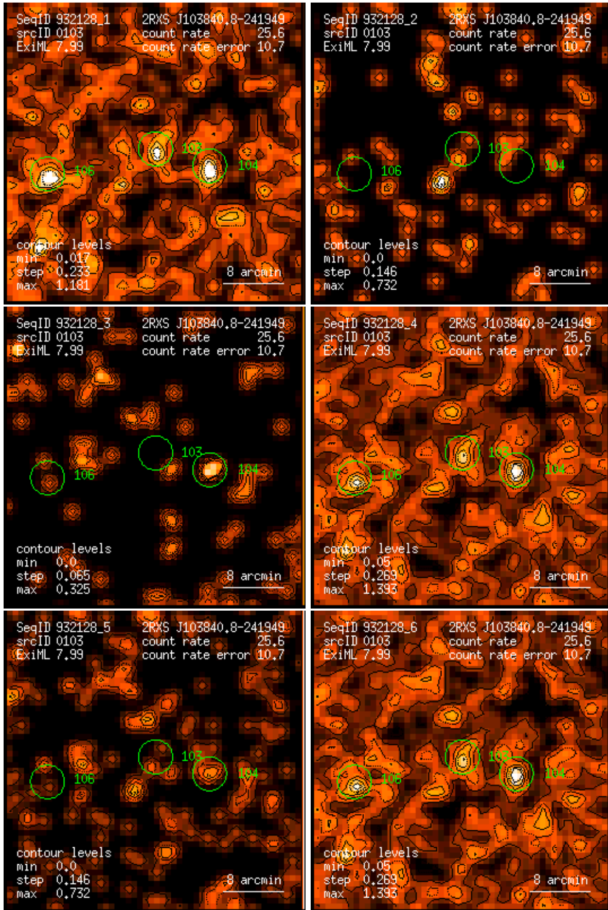
Figure 103: RASS 932128: detection 0103: band rate images, Gaussian filter: (1) PSPC channels 11 – 41, (2) 52 – 90, (3) 91 – 201, (4) 11 – 235, (5) 52 – 201, (6) 11 – 201. Broad band rates in counts/ks. Band rate contour levels in counts/ks/arcmin 2 .
