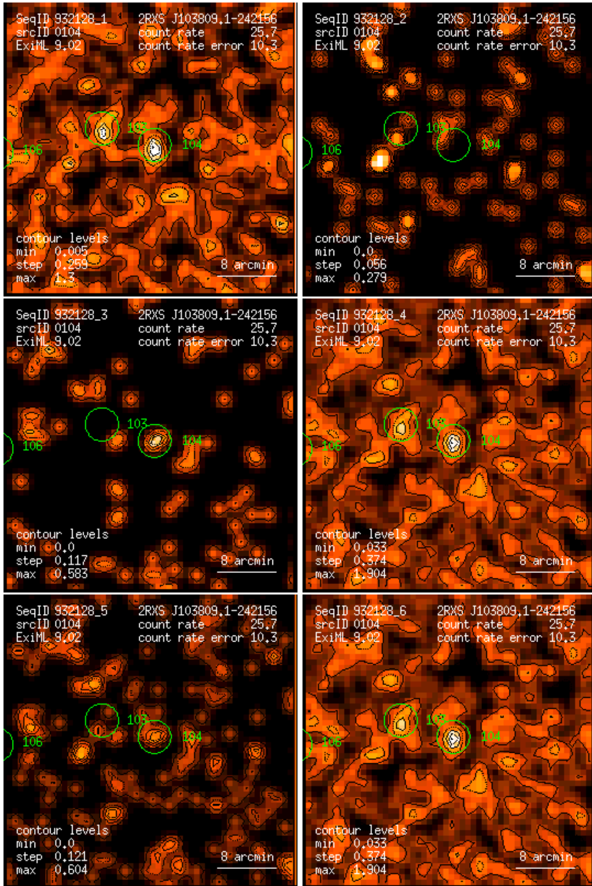
Figure 104: RASS 932128: detection 0104: band rate images, Gaussian filter: (1) PSPC channels 11 – 41, (2) 52 – 90, (3) 91 – 201, (4) 11 – 235, (5) 52 – 201, (6) 11 – 201. Broad band rates in counts/ks. Band rate contour levels in counts/ks/arcmin 2 .
