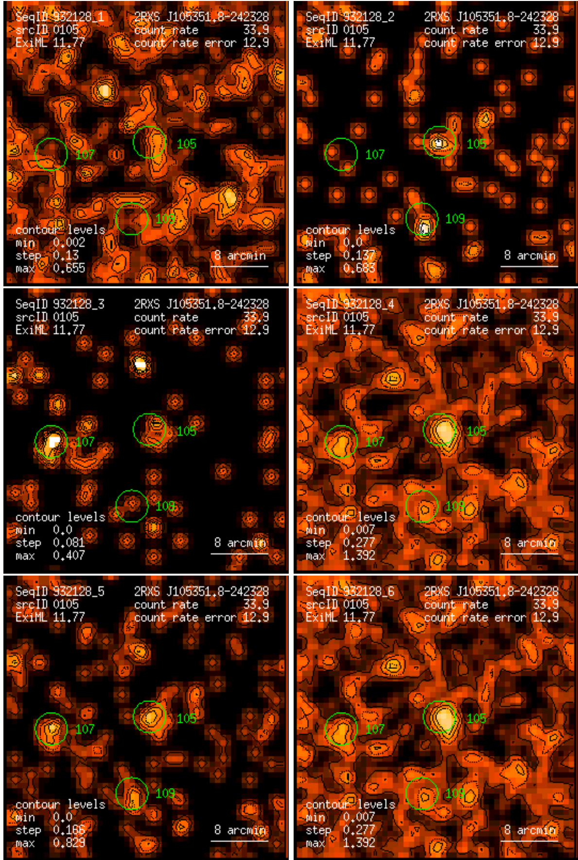
Figure 105: RASS 932128: detection 0105: band rate images, Gaussian filter: (1) PSPC channels 11 – 41, (2) 52 – 90, (3) 91 – 201, (4) 11 – 235, (5) 52 – 201, (6) 11 – 201. Broad band rates in counts/ks. Band rate contour levels in counts/ks/arcmin 2 .
