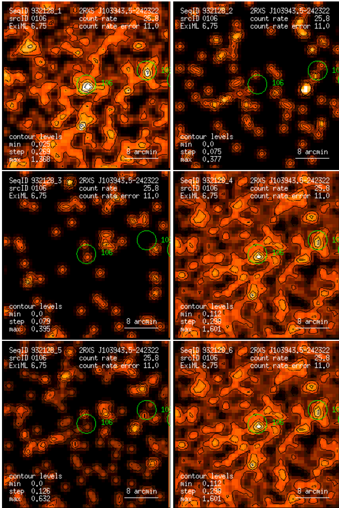
Figure 106: RASS 932128: detection 0106: band rate images, Gaussian filter: (1) PSPC channels 11 – 41, (2) 52 – 90, (3) 91 – 201, (4) 11 – 235, (5) 52 – 201, (6) 11 – 201. Broad band rates in counts/ks. Band rate contour levels in counts/ks/arcmin 2 .
