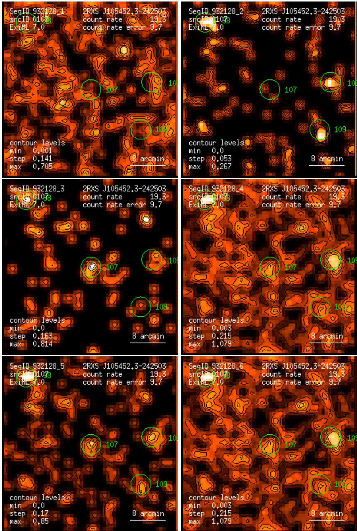
Figure 107: RASS 932128: detection 0107: band rate images, Gaussian filter: (1) PSPC channels 11 – 41, (2) 52 – 90, (3) 91 – 201, (4) 11 – 235, (5) 52 – 201, (6) 11 – 201. Broad band rates in counts/ks. Band rate contour levels in counts/ks/arcmin 2 .
