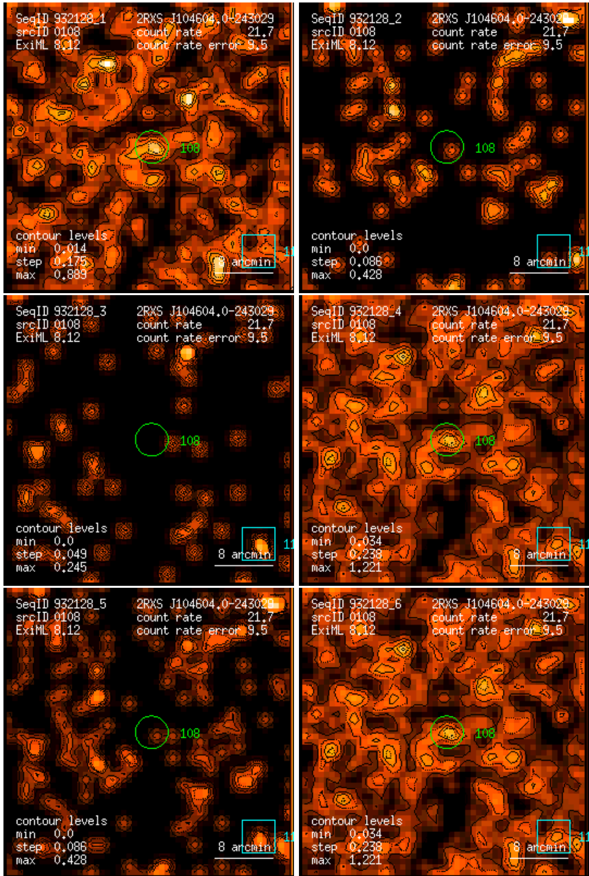
Figure 108: RASS 932128: detection 0108: band rate images, Gaussian filter: (1) PSPC channels 11 – 41, (2) 52 – 90, (3) 91 – 201, (4) 11 – 235, (5) 52 – 201, (6) 11 – 201. Broad band rates in counts/ks. Band rate contour levels in counts/ks/arcmin 2 .
