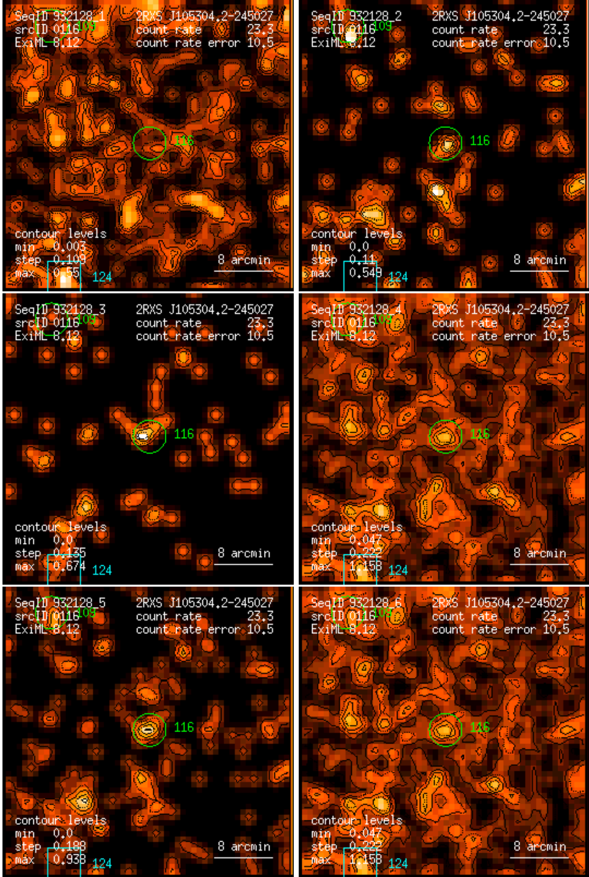
Figure 116: RASS 932128: detection 0116: band rate images, Gaussian filter: (1) PSPC channels 11 – 41, (2) 52 – 90, (3) 91 – 201, (4) 11 – 235, (5) 52 – 201, (6) 11 – 201. Broad band rates in counts/ks. Band rate contour levels in counts/ks/arcmin 2 .
