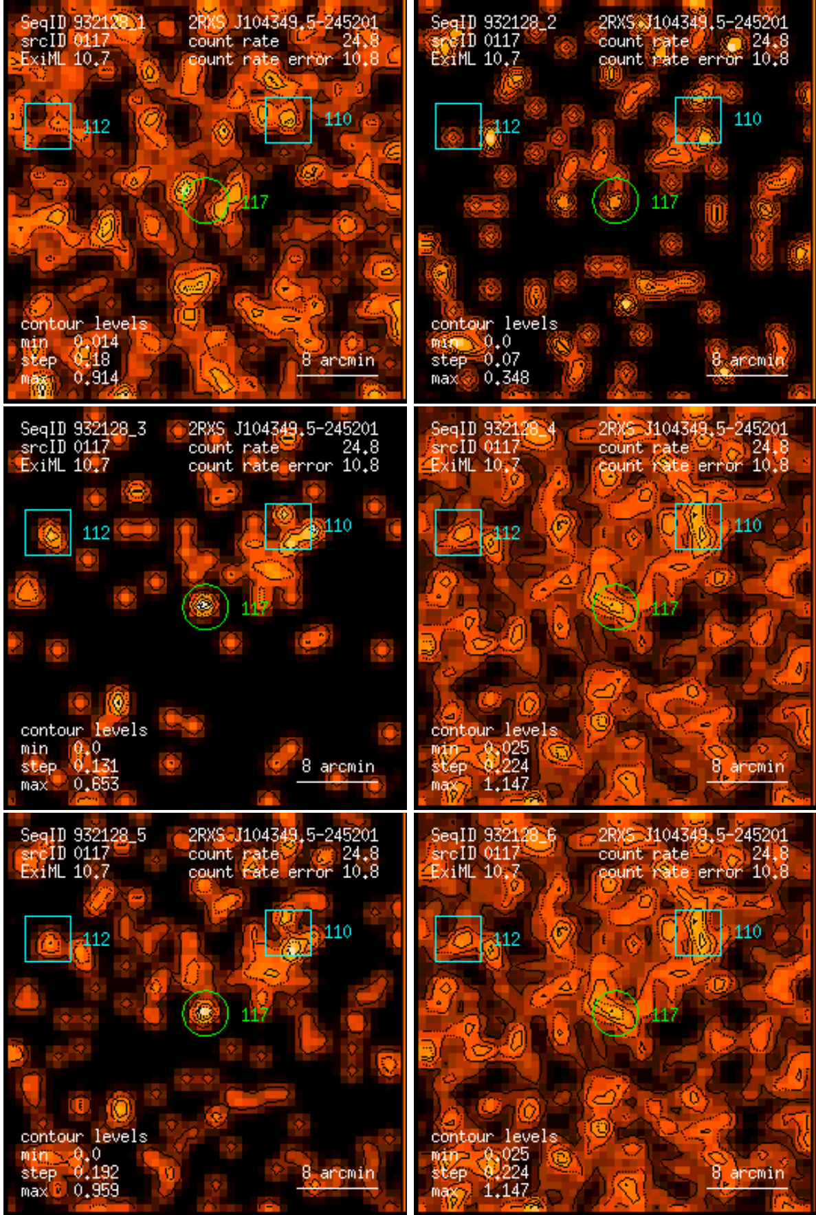
Figure 117: RASS 932128: detection 0117: band rate images, Gaussian filter: (1) PSPC channels 11 – 41, (2) 52 – 90, (3) 91 – 201, (4) 11 – 235, (5) 52 – 201, (6) 11 – 201. Broad band rates in counts/ks. Band rate contour levels in counts/ks/arcmin 2 .
