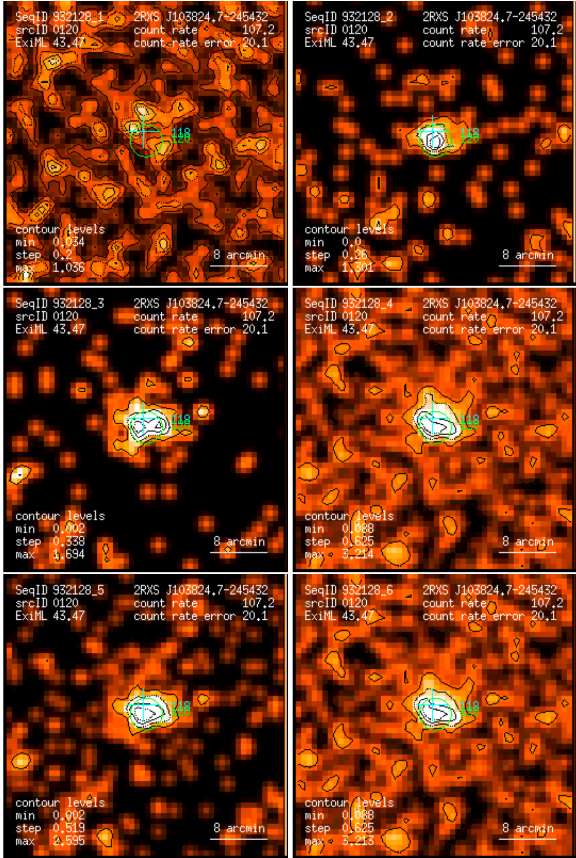
Figure 120: RASS 932128: detection 0120: band rate images, Gaussian filter: (1) PSPC channels 11 – 41, (2) 52 – 90, (3) 91 – 201, (4) 11 – 235, (5) 52 – 201, (6) 11 – 201. Broad band rates in counts/ks. Band rate contour levels in counts/ks/arcmin 2 .
