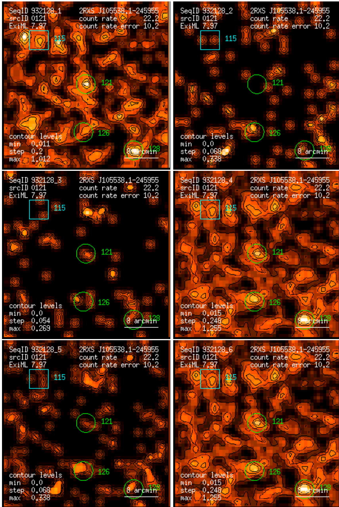
Figure 121: RASS 932128: detection 0121: band rate images, Gaussian filter: (1) PSPC channels 11 – 41, (2) 52 – 90, (3) 91 – 201, (4) 11 – 235, (5) 52 – 201, (6) 11 – 201. Broad band rates in counts/ks. Band rate contour levels in counts/ks/arcmin 2 .
