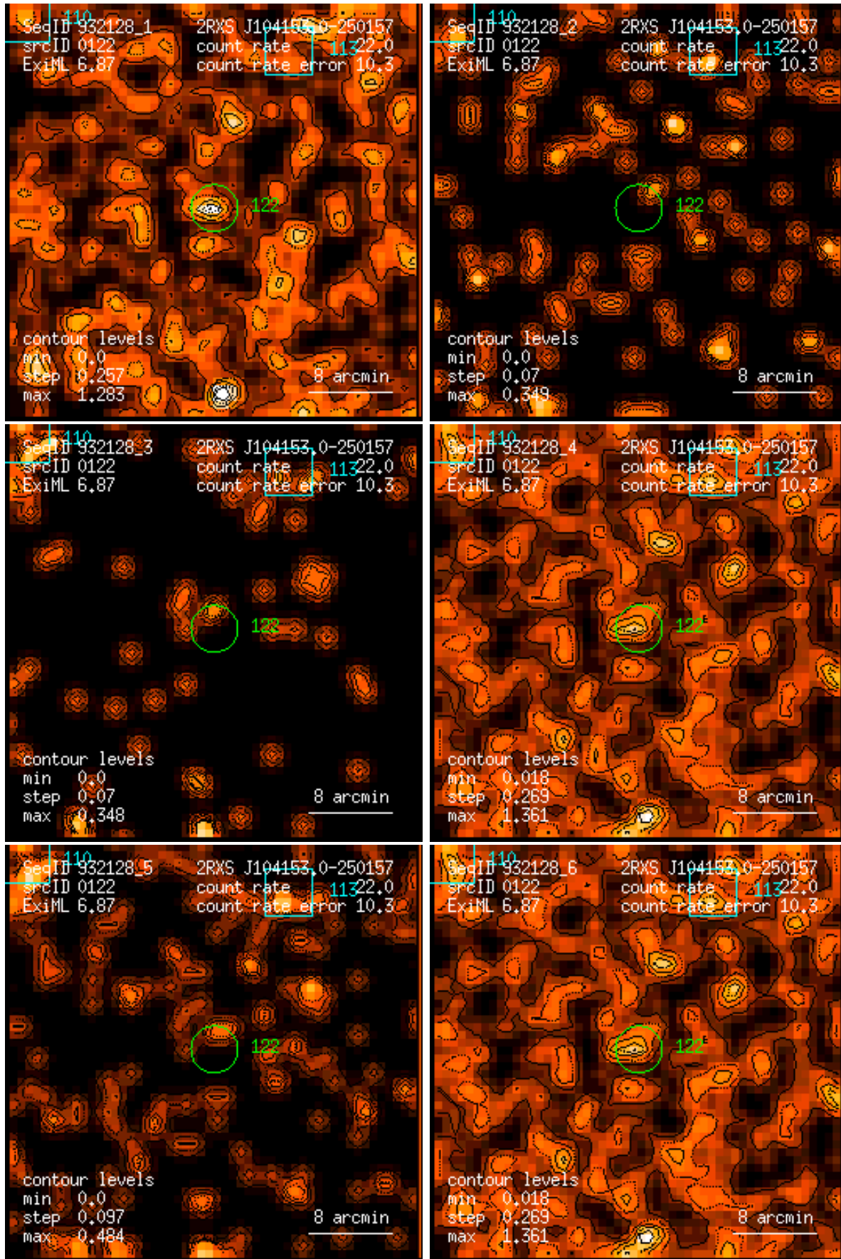
Figure 122: RASS 932128: detection 0122: band rate images, Gaussian filter: (1) PSPC channels 11 – 41, (2) 52 – 90, (3) 91 – 201, (4) 11 – 235, (5) 52 – 201, (6) 11 – 201. Broad band rates in counts/ks. Band rate contour levels in counts/ks/arcmin 2 .
