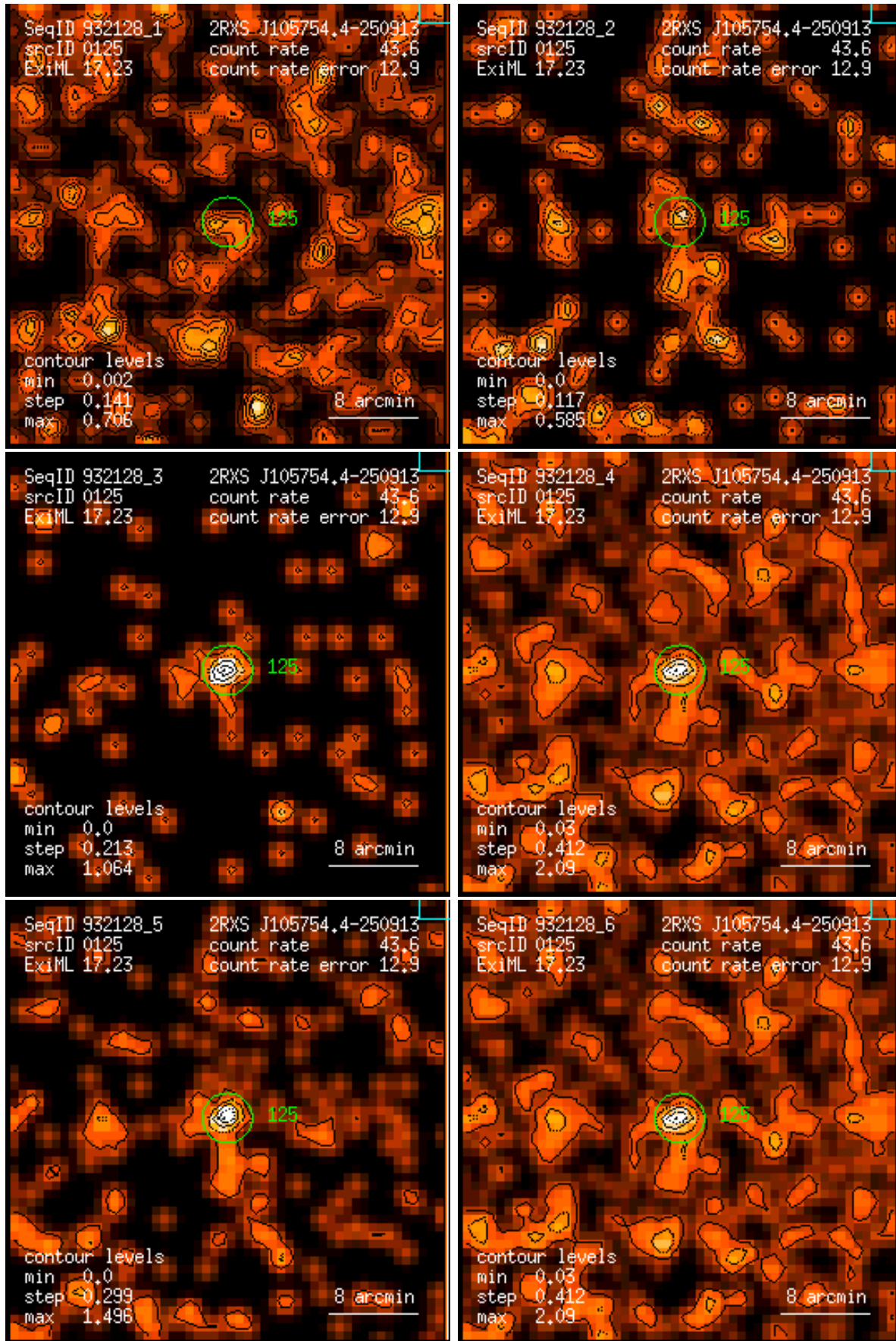
Figure 125: RASS 932128: detection 0125: band rate images, Gaussian filter: (1) PSPC channels 11 – 41, (2) 52 – 90, (3) 91 – 201, (4) 11 – 235, (5) 52 – 201, (6) 11 – 201. Broad band rates in counts/ks. Band rate contour levels in counts/ks/arcmin 2 .
