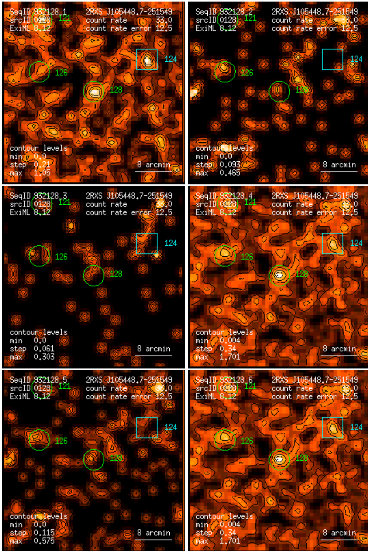
Figure 128: RASS 932128: detection 0128: band rate images, Gaussian filter: (1) PSPC channels 11 – 41, (2) 52 – 90, (3) 91 – 201, (4) 11 – 235, (5) 52 – 201, (6) 11 – 201. Broad band rates in counts/ks. Band rate contour levels in counts/ks/arcmin 2 .
