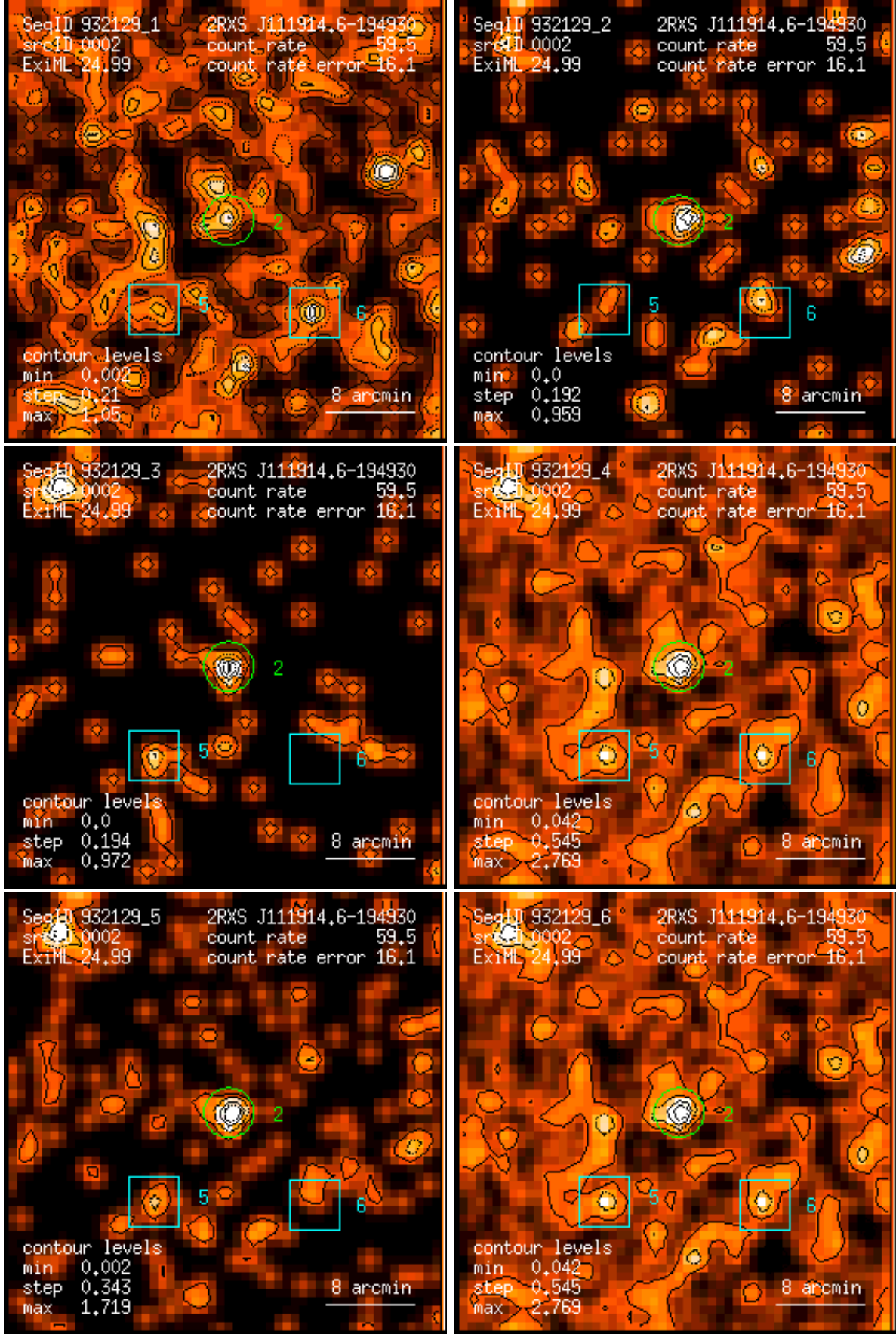
Figure 2: RASS 932129: detection 0002: band rate images, Gaussian filter: (1) PSPC channels 11 – 41, (2) 52 – 90, (3) 91 – 201, (4) 11 – 235, (5) 52 – 201, (6) 11 – 201. Broad band rates in counts/ks. Band rate contour levels in counts/ks/arcmin 2 .
