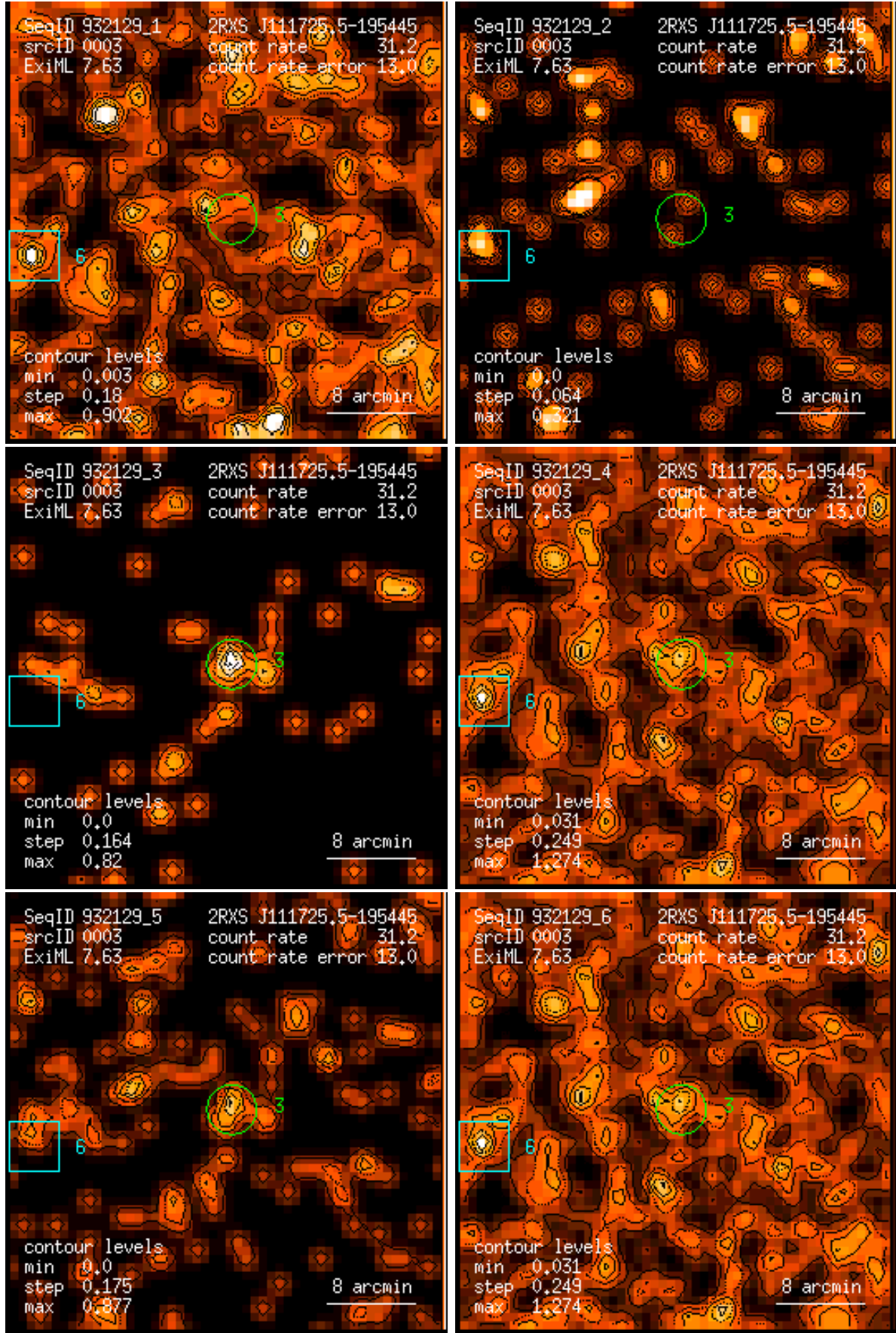
Figure 3: RASS 932129: detection 0003: band rate images, Gaussian filter: (1) PSPC channels 11 – 41, (2) 52 – 90, (3) 91 – 201, (4) 11 – 235, (5) 52 – 201, (6) 11 – 201. Broad band rates in counts/ks. Band rate contour levels in counts/ks/arcmin 2 .
