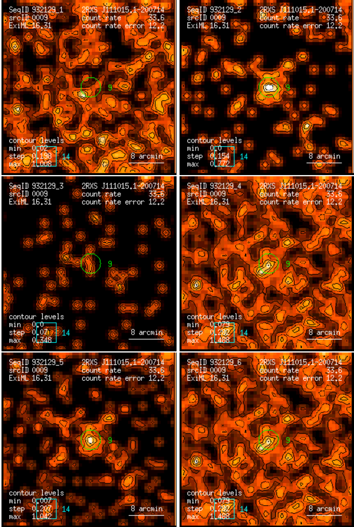
Figure 9: RASS 932129: detection 0009: band rate images, Gaussian filter: (1) PSPC channels 11 – 41, (2) 52 – 90, (3) 91 – 201, (4) 11 – 235, (5) 52 – 201, (6) 11 – 201. Broad band rates in counts/ks. Band rate contour levels in counts/ks/arcmin 2 .
