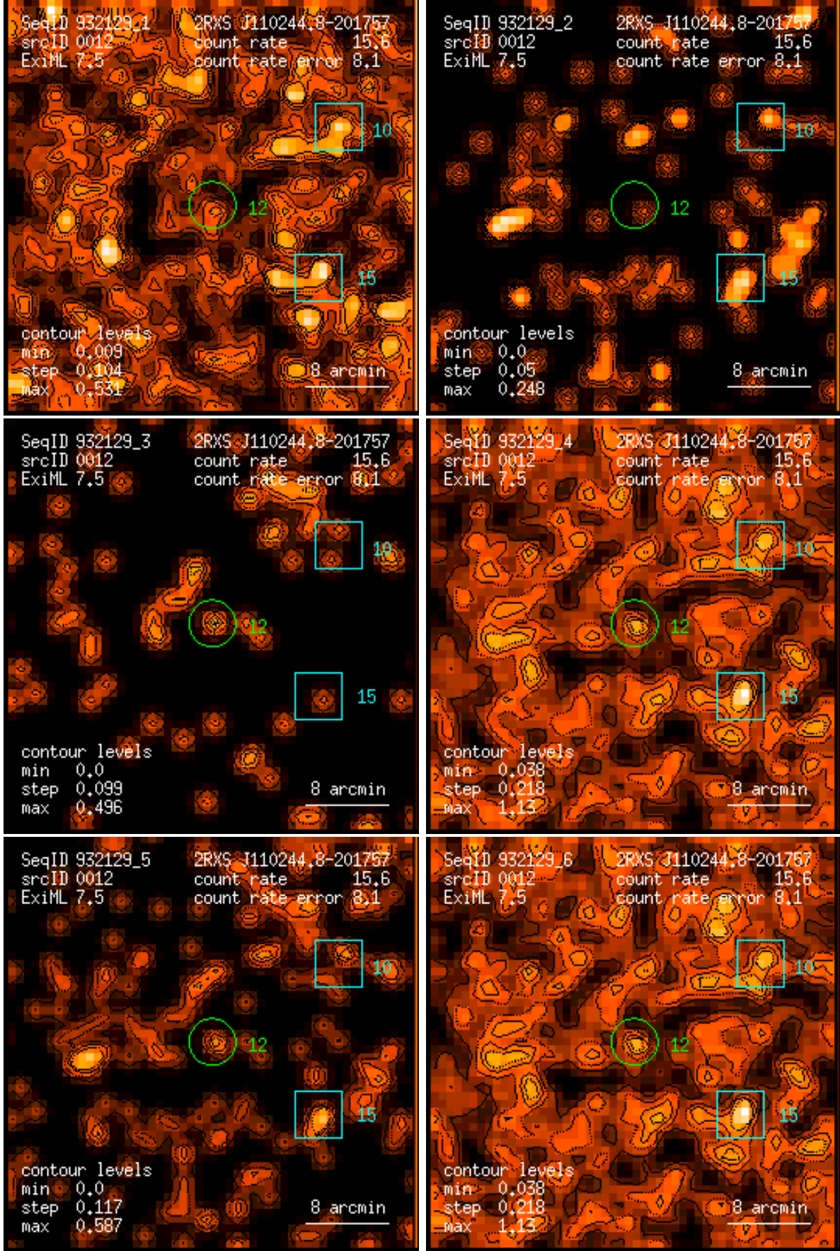
Figure 12: RASS 932129: detection 0012: band rate images, Gaussian filter: (1) PSPC channels 11 – 41, (2) 52 – 90, (3) 91 – 201, (4) 11 – 235, (5) 52 – 201, (6) 11 – 201. Broad band rates in counts/ks. Band rate contour levels in counts/ks/arcmin 2 .
