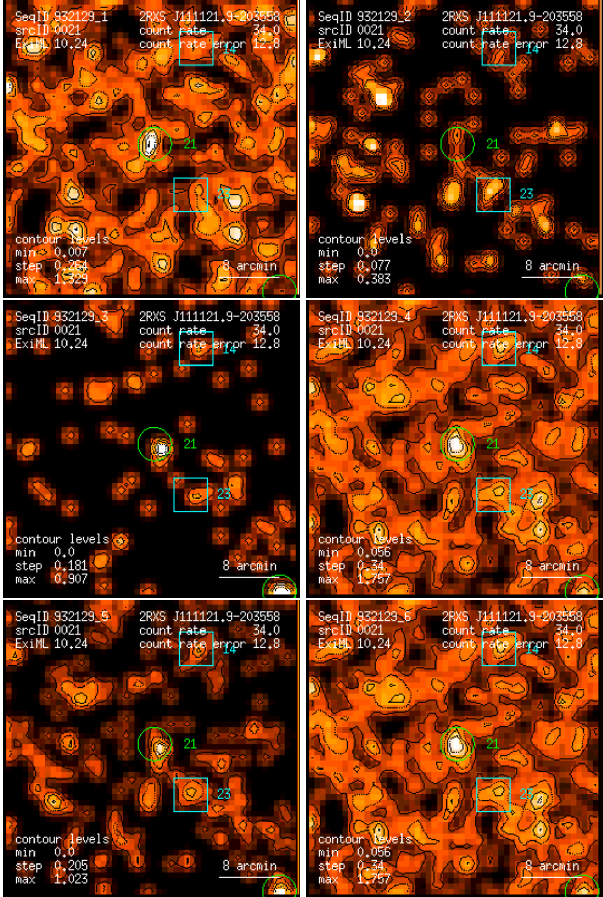
Figure 21: RASS 932129: detection 0021: band rate images, Gaussian filter: (1) PSPC channels 11 – 41, (2) 52 – 90, (3) 91 – 201, (4) 11 – 235, (5) 52 – 201, (6) 11 – 201. Broad band rates in counts/ks. Band rate contour levels in counts/ks/arcmin 2 .
