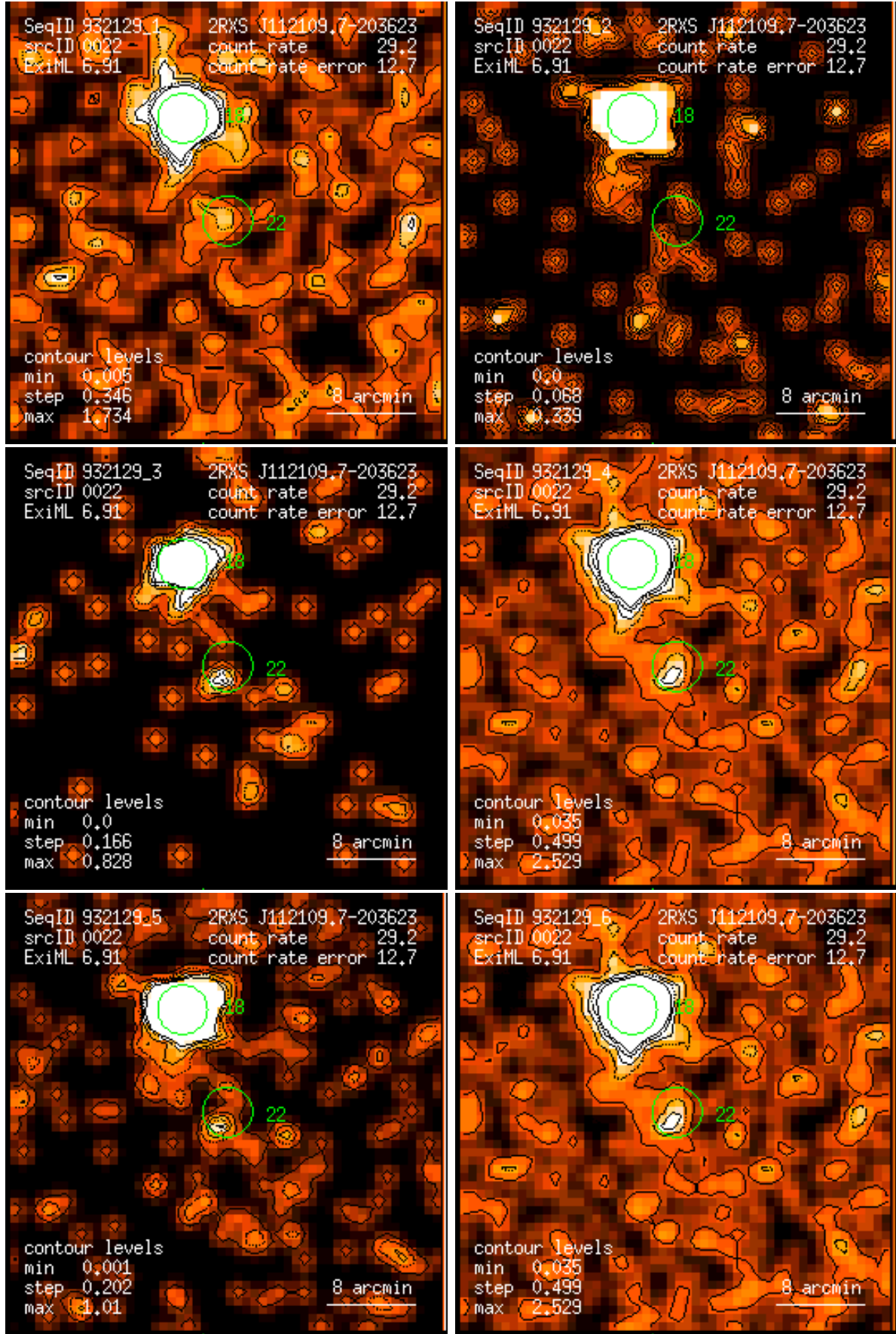
Figure 22: RASS 932129: detection 0022: band rate images, Gaussian filter: (1) PSPC channels 11 – 41, (2) 52 – 90, (3) 91 – 201, (4) 11 – 235, (5) 52 – 201, (6) 11 – 201. Broad band rates in counts/ks. Band rate contour levels in counts/ks/arcmin 2 .
