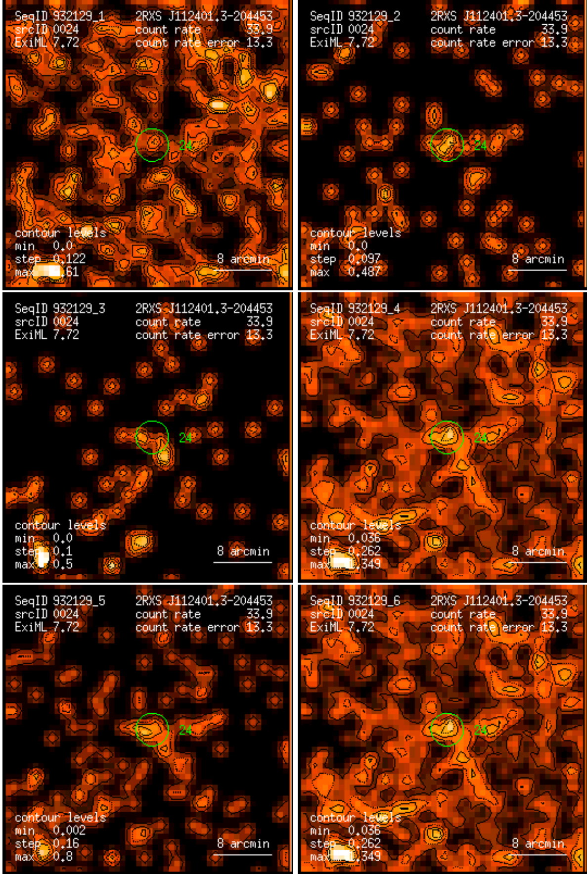
Figure 24: RASS 932129: detection 0024: band rate images, Gaussian filter: (1) PSPC channels 11 – 41, (2) 52 – 90, (3) 91 – 201, (4) 11 – 235, (5) 52 – 201, (6) 11 – 201. Broad band rates in counts/ks. Band rate contour levels in counts/ks/arcmin 2 .
