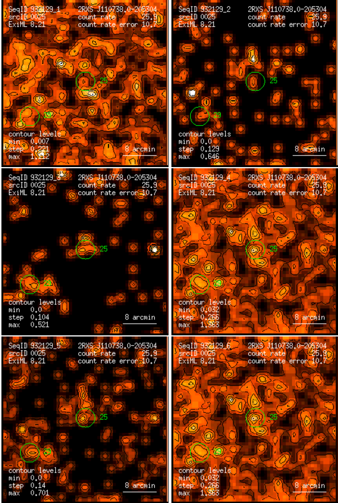
Figure 25: RASS 932129: detection 0025: band rate images, Gaussian filter: (1) PSPC channels 11 – 41, (2) 52 – 90, (3) 91 – 201, (4) 11 – 235, (5) 52 – 201, (6) 11 – 201. Broad band rates in counts/ks. Band rate contour levels in counts/ks/arcmin 2 .
