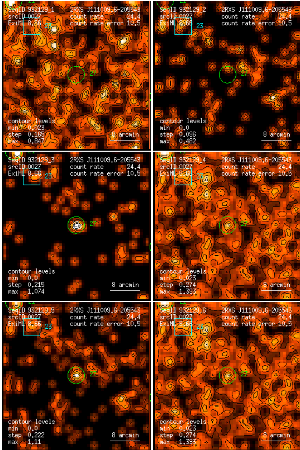
Figure 27: RASS 932129: detection 0027: band rate images, Gaussian filter: (1) PSPC channels 11 – 41, (2) 52 – 90, (3) 91 – 201, (4) 11 – 235, (5) 52 – 201, (6) 11 – 201. Broad band rates in counts/ks. Band rate contour levels in counts/ks/arcmin 2 .
