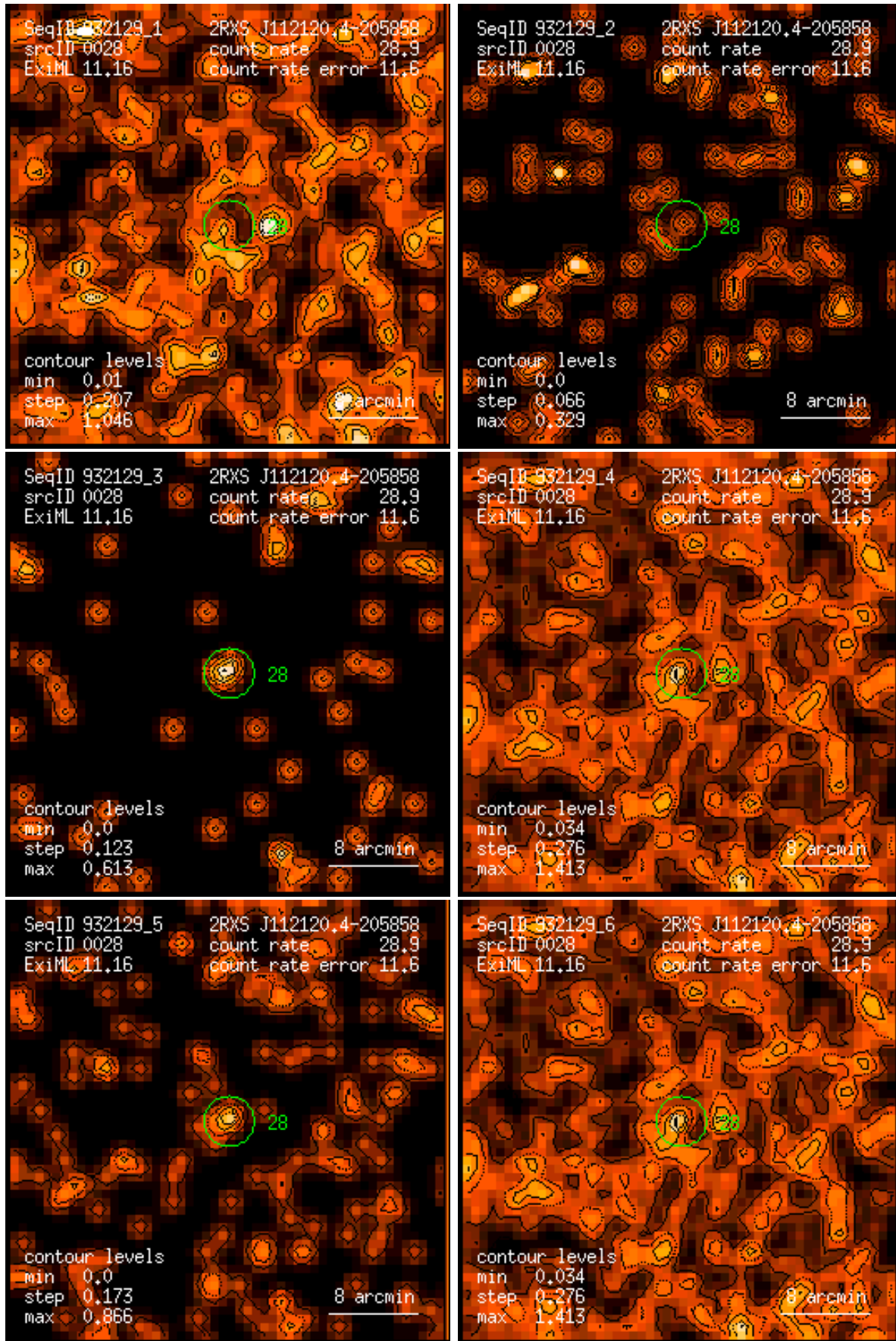
Figure 28: RASS 932129: detection 0028: band rate images, Gaussian filter: (1) PSPC channels 11 – 41, (2) 52 – 90, (3) 91 – 201, (4) 11 – 235, (5) 52 – 201, (6) 11 – 201. Broad band rates in counts/ks. Band rate contour levels in counts/ks/arcmin 2 .
