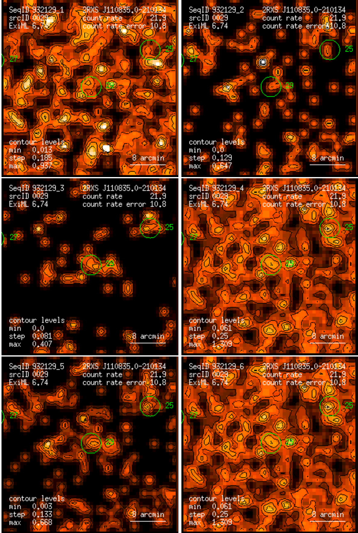
Figure 29: RASS 932129: detection 0029: band rate images, Gaussian filter: (1) PSPC channels 11 – 41, (2) 52 – 90, (3) 91 – 201, (4) 11 – 235, (5) 52 – 201, (6) 11 – 201. Broad band rates in counts/ks. Band rate contour levels in counts/ks/arcmin 2 .
