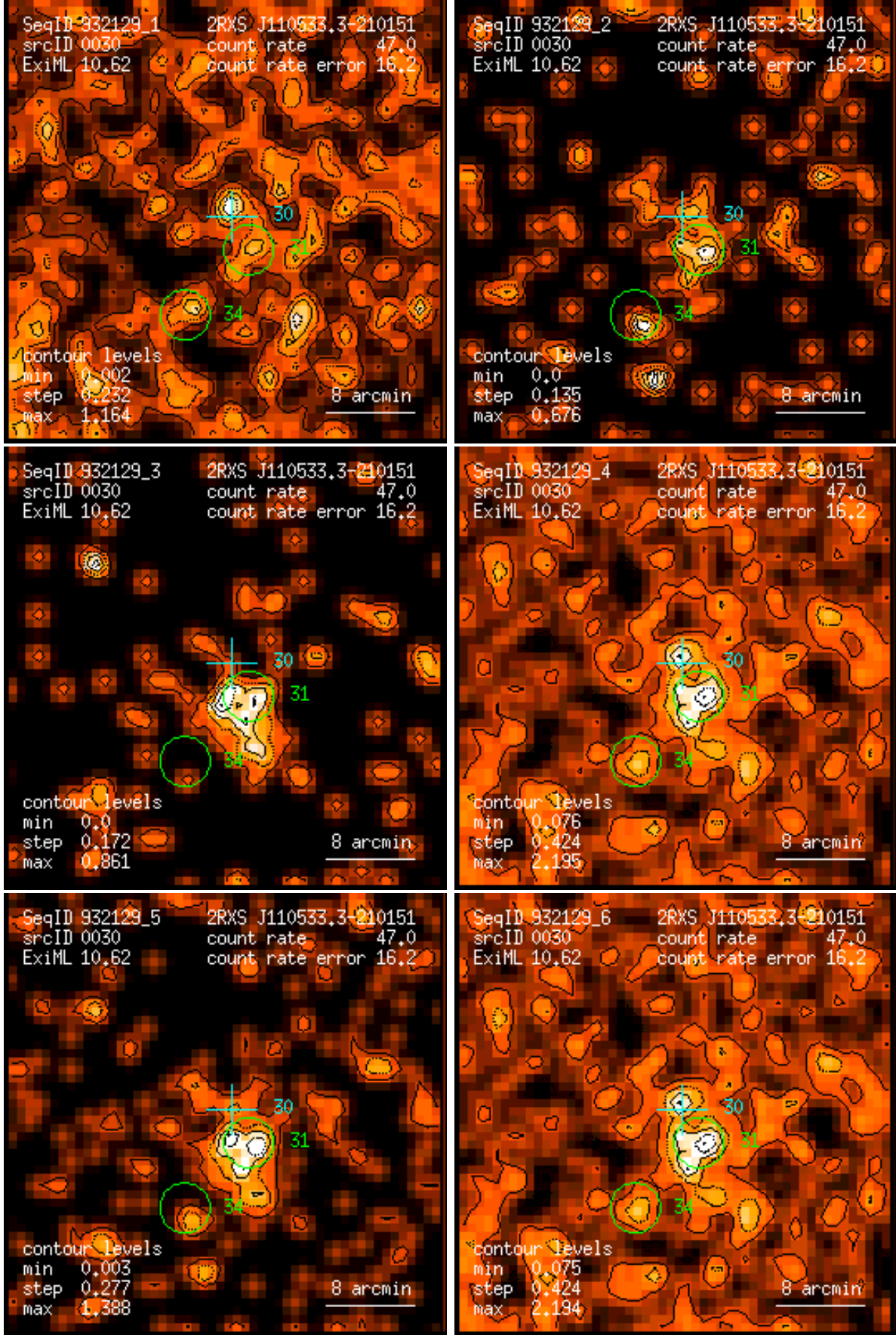
Figure 30: RASS 932129: detection 0030: band rate images, Gaussian filter: (1) PSPC channels 11 – 41, (2) 52 – 90, (3) 91 – 201, (4) 11 – 235, (5) 52 – 201, (6) 11 – 201. Broad band rates in counts/ks. Band rate contour levels in counts/ks/arcmin 2 .
