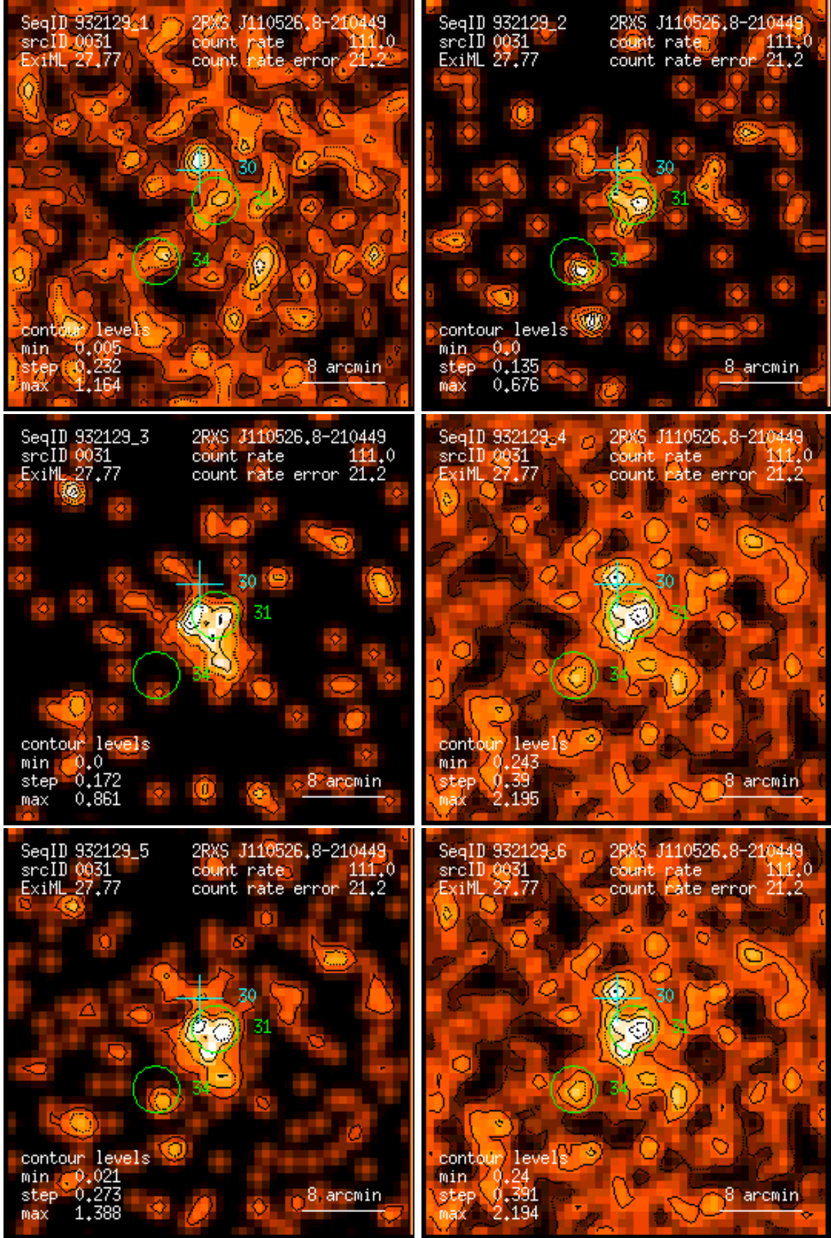
Figure 31: RASS 932129: detection 0031: band rate images, Gaussian filter: (1) PSPC channels 11 – 41, (2) 52 – 90, (3) 91 – 201, (4) 11 – 235, (5) 52 – 201, (6) 11 – 201. Broad band rates in counts/ks. Band rate contour levels in counts/ks/arcmin 2 .
