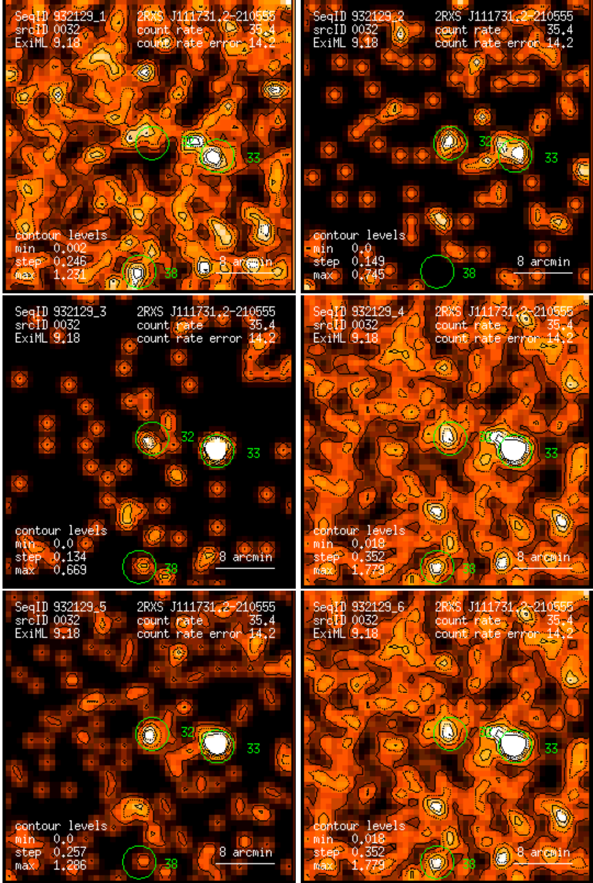
Figure 32: RASS 932129: detection 0032: band rate images, Gaussian filter: (1) PSPC channels 11 – 41, (2) 52 – 90, (3) 91 – 201, (4) 11 – 235, (5) 52 – 201, (6) 11 – 201. Broad band rates in counts/ks. Band rate contour levels in counts/ks/arcmin 2 .
