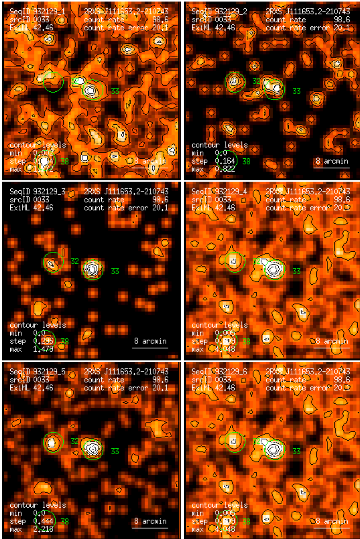
Figure 33: RASS 932129: detection 0033: band rate images, Gaussian filter: (1) PSPC channels 11 – 41, (2) 52 – 90, (3) 91 – 201, (4) 11 – 235, (5) 52 – 201, (6) 11 – 201. Broad band rates in counts/ks. Band rate contour levels in counts/ks/arcmin 2 .
