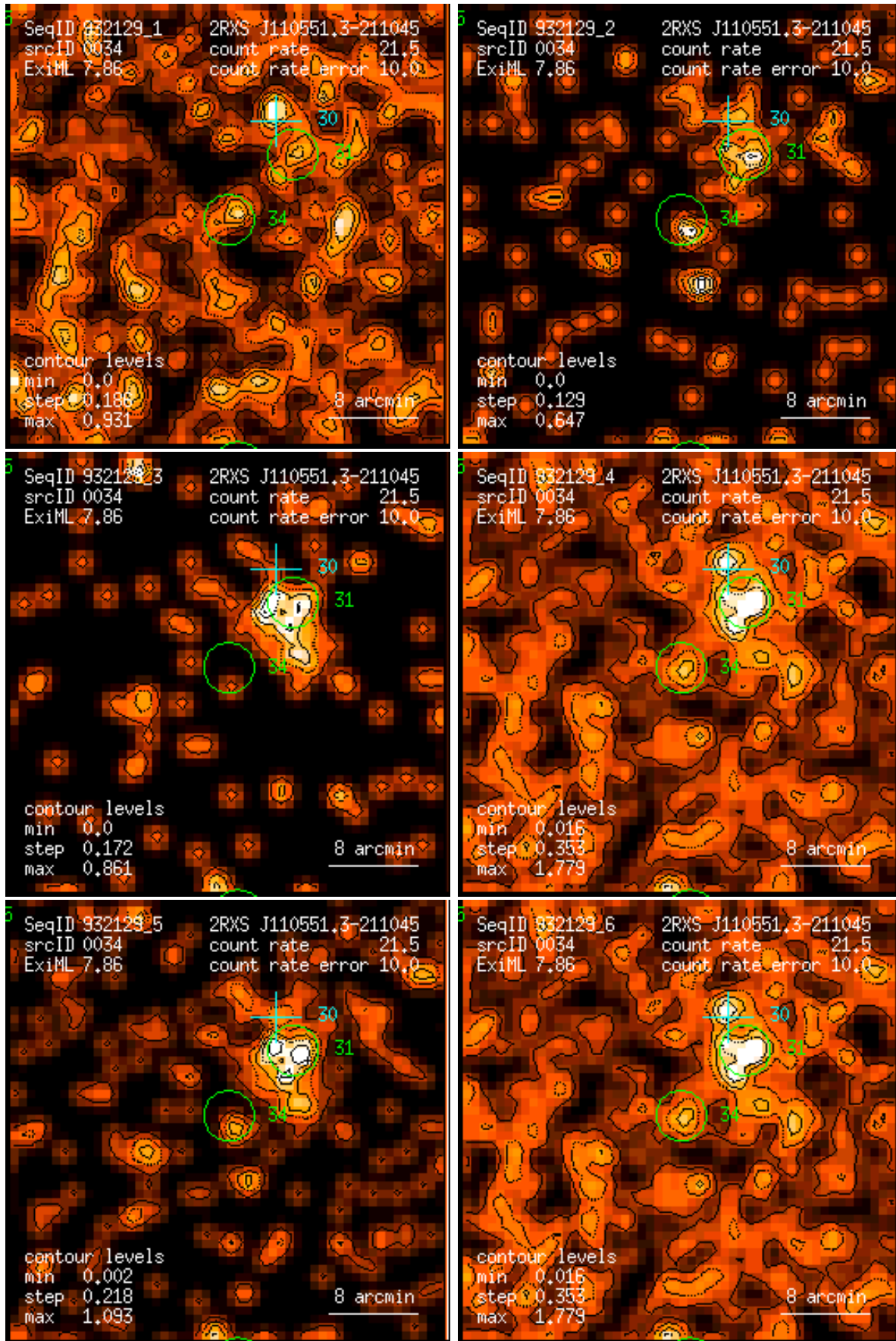
Figure 34: RASS 932129: detection 0034: band rate images, Gaussian filter: (1) PSPC channels 11 – 41, (2) 52 – 90, (3) 91 – 201, (4) 11 – 235, (5) 52 – 201, (6) 11 – 201. Broad band rates in counts/ks. Band rate contour levels in counts/ks/arcmin 2 .
