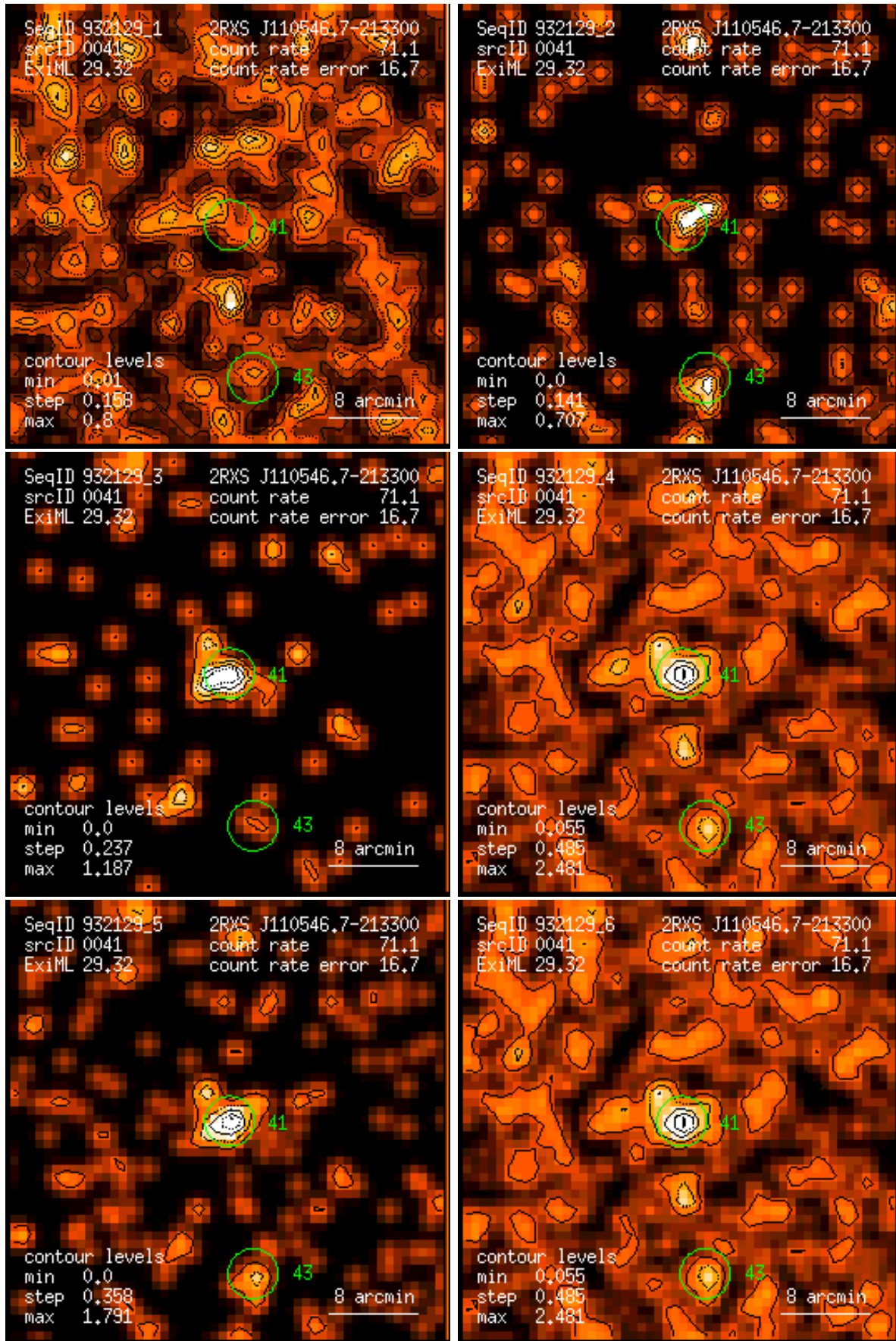
Figure 41: RASS 932129: detection 0041: band rate images, Gaussian filter: (1) PSPC channels 11 – 41, (2) 52 – 90, (3) 91 – 201, (4) 11 – 235, (5) 52 – 201, (6) 11 – 201. Broad band rates in counts/ks. Band rate contour levels in counts/ks/arcmin 2 .
