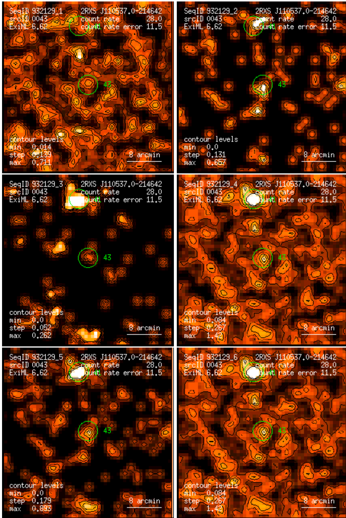
Figure 43: RASS 932129: detection 0043: band rate images, Gaussian filter: (1) PSPC channels 11 – 41, (2) 52 – 90, (3) 91 – 201, (4) 11 – 235, (5) 52 – 201, (6) 11 – 201. Broad band rates in counts/ks. Band rate contour levels in counts/ks/arcmin 2 .
