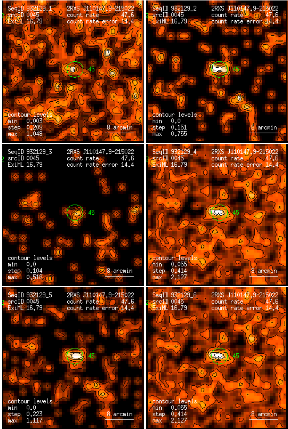
Figure 45: RASS 932129: detection 0045: band rate images, Gaussian filter: (1) PSPC channels 11 – 41, (2) 52 – 90, (3) 91 – 201, (4) 11 – 235, (5) 52 – 201, (6) 11 – 201. Broad band rates in counts/ks. Band rate contour levels in counts/ks/arcmin 2 .
