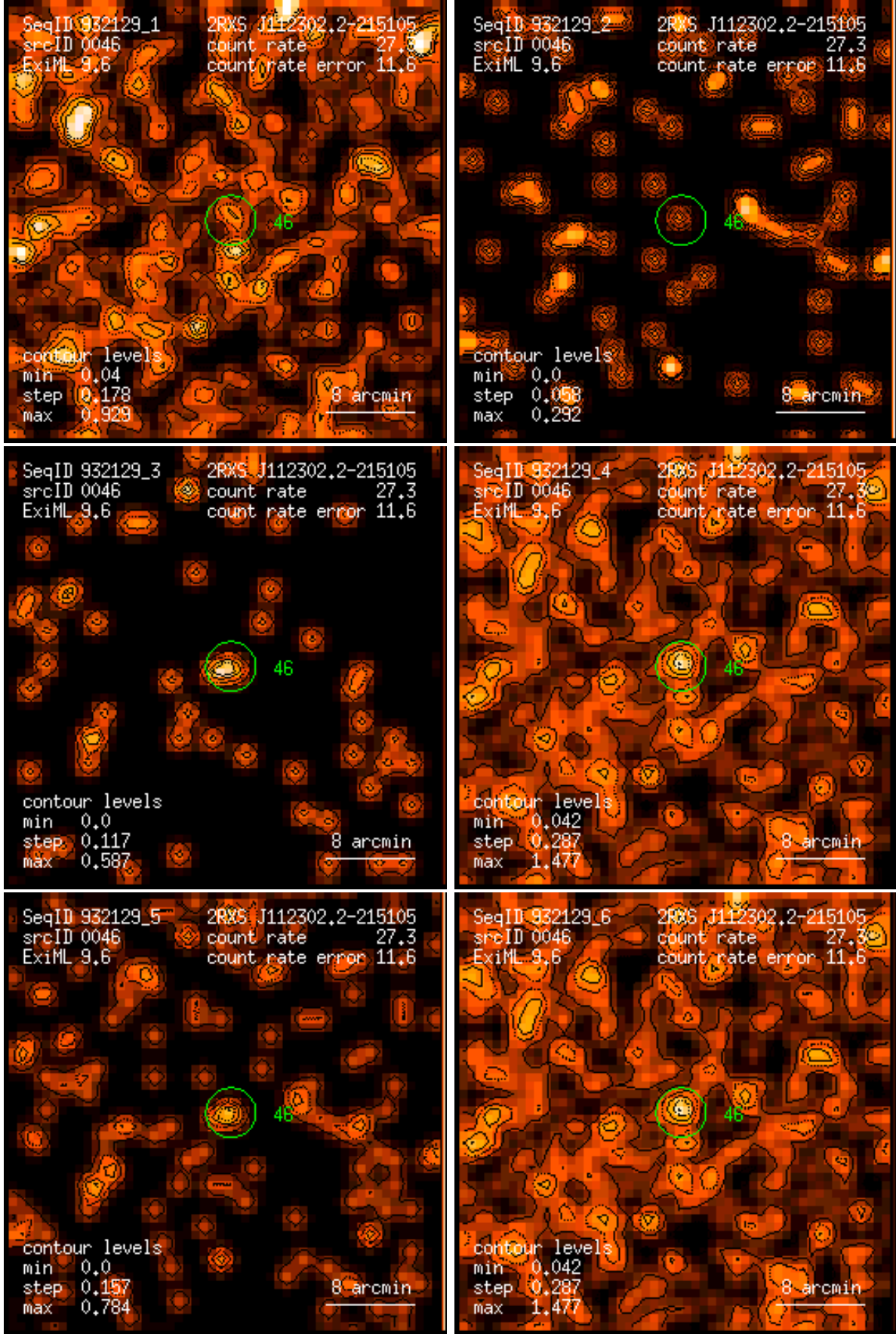
Figure 46: RASS 932129: detection 0046: band rate images, Gaussian filter: (1) PSPC channels 11 – 41, (2) 52 – 90, (3) 91 – 201, (4) 11 – 235, (5) 52 – 201, (6) 11 – 201. Broad band rates in counts/ks. Band rate contour levels in counts/ks/arcmin 2 .
