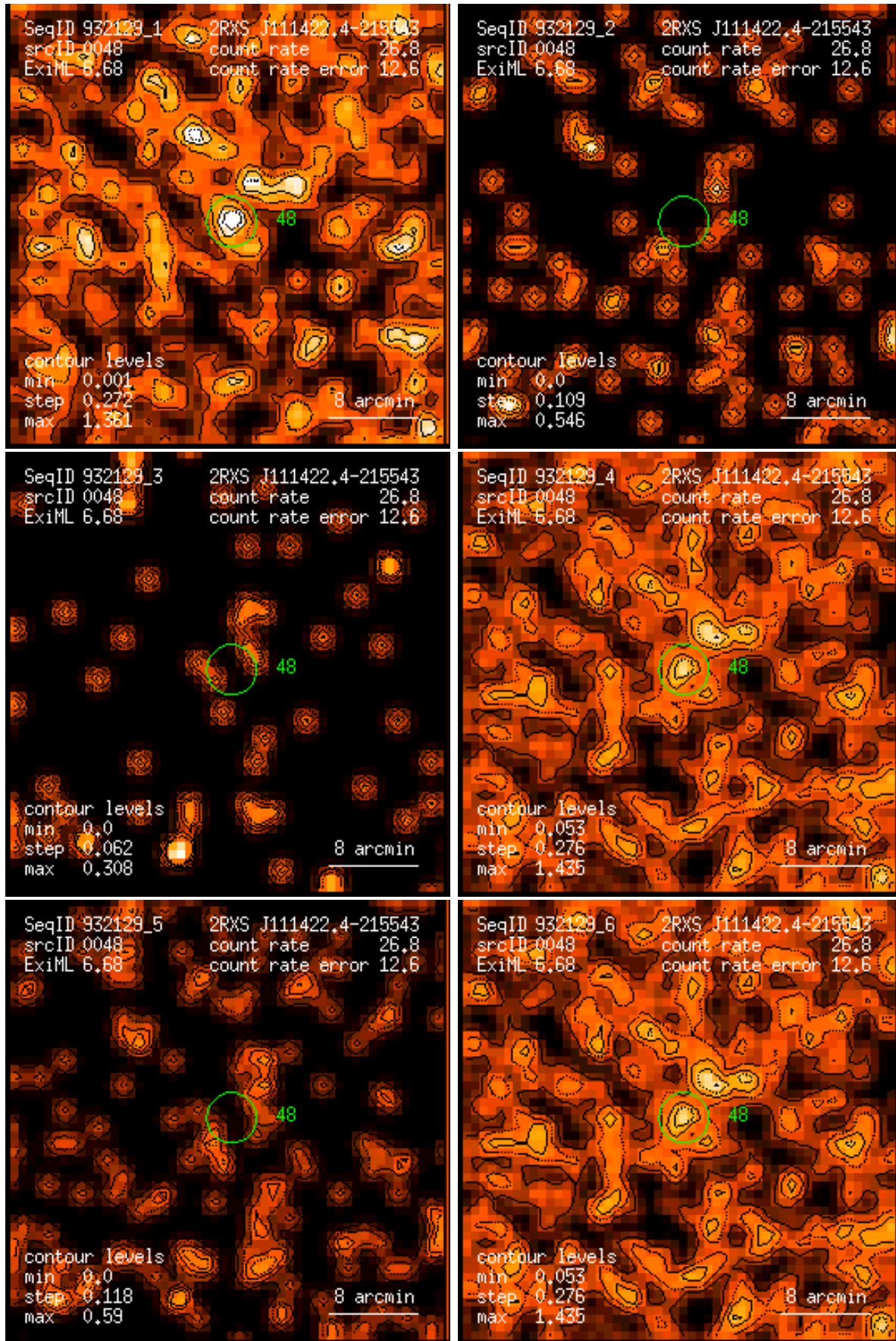
Figure 48: RASS 932129: detection 0048: band rate images, Gaussian filter: (1) PSPC channels 11 – 41, (2) 52 – 90, (3) 91 – 201, (4) 11 – 235, (5) 52 – 201, (6) 11 – 201. Broad band rates in counts/ks. Band rate contour levels in counts/ks/arcmin 2 .
