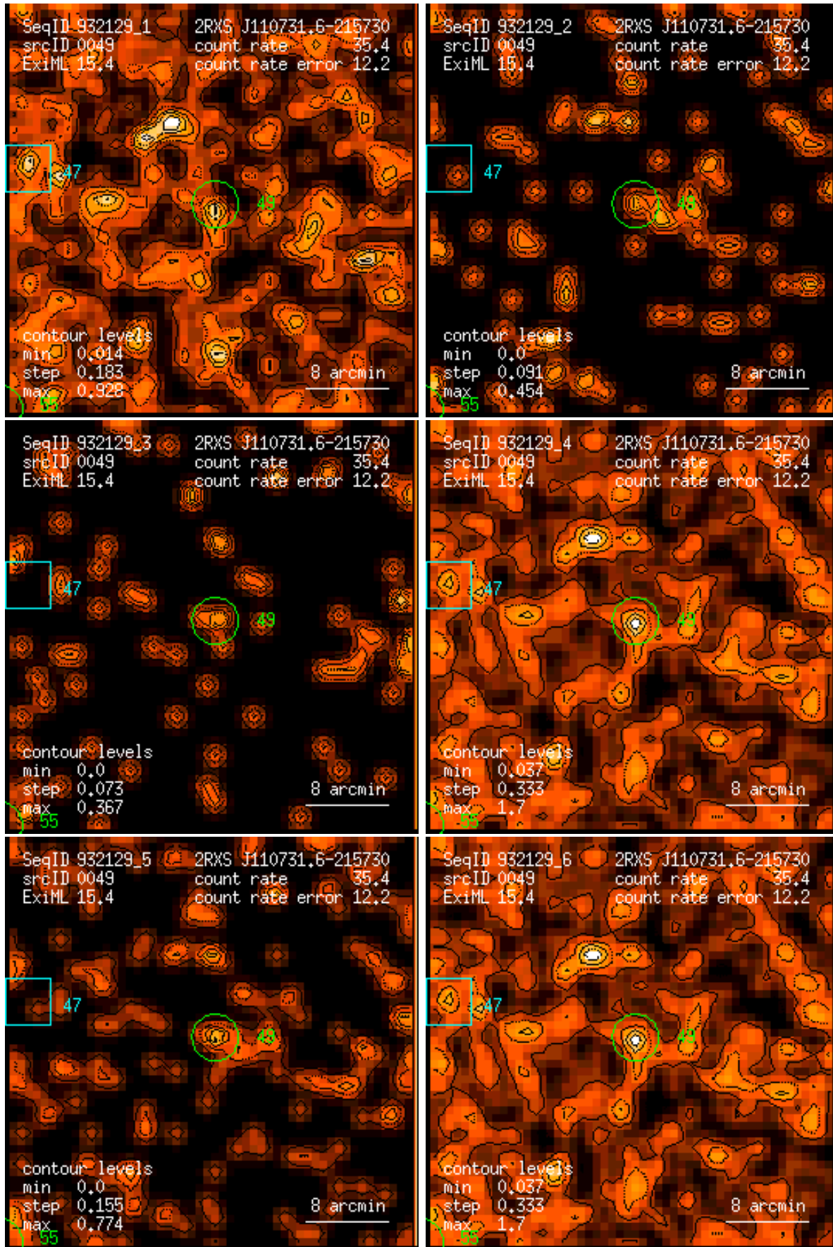
Figure 49: RASS 932129: detection 0049: band rate images, Gaussian filter: (1) PSPC channels 11 – 41, (2) 52 – 90, (3) 91 – 201, (4) 11 – 235, (5) 52 – 201, (6) 11 – 201. Broad band rates in counts/ks. Band rate contour levels in counts/ks/arcmin 2 .
