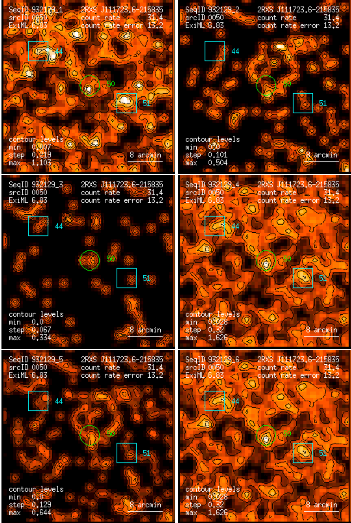
Figure 50: RASS 932129: detection 0050: band rate images, Gaussian filter: (1) PSPC channels 11 – 41, (2) 52 – 90, (3) 91 – 201, (4) 11 – 235, (5) 52 – 201, (6) 11 – 201. Broad band rates in counts/ks. Band rate contour levels in counts/ks/arcmin 2 .
