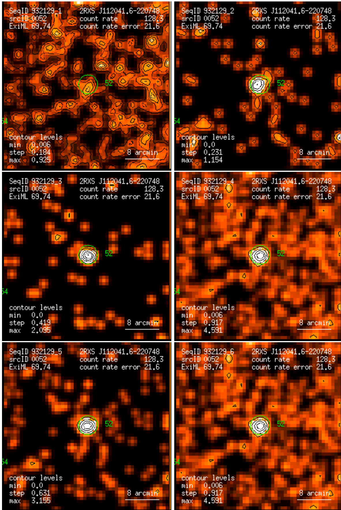
Figure 52: RASS 932129: detection 0052: band rate images, Gaussian filter: (1) PSPC channels 11 – 41, (2) 52 – 90, (3) 91 – 201, (4) 11 – 235, (5) 52 – 201, (6) 11 – 201. Broad band rates in counts/ks. Band rate contour levels in counts/ks/arcmin 2 .
