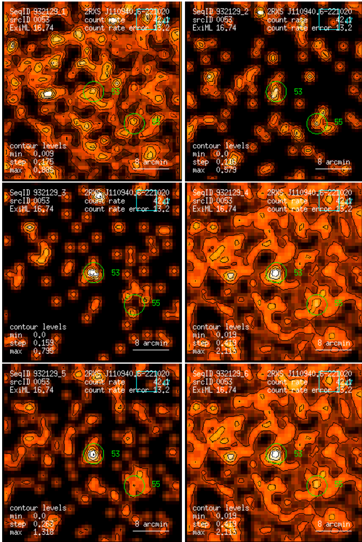
Figure 53: RASS 932129: detection 0053: band rate images, Gaussian filter: (1) PSPC channels 11 – 41, (2) 52 – 90, (3) 91 – 201, (4) 11 – 235, (5) 52 – 201, (6) 11 – 201. Broad band rates in counts/ks. Band rate contour levels in counts/ks/arcmin 2 .
