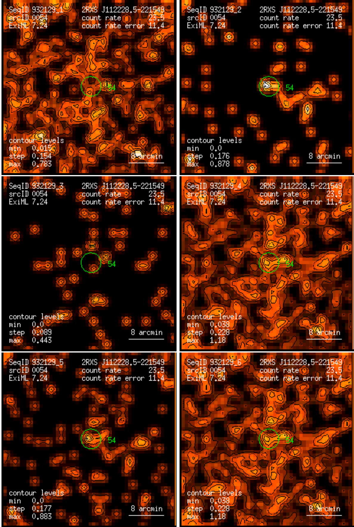
Figure 54: RASS 932129: detection 0054: band rate images, Gaussian filter: (1) PSPC channels 11 – 41, (2) 52 – 90, (3) 91 – 201, (4) 11 – 235, (5) 52 – 201, (6) 11 – 201. Broad band rates in counts/ks. Band rate contour levels in counts/ks/arcmin 2 .
