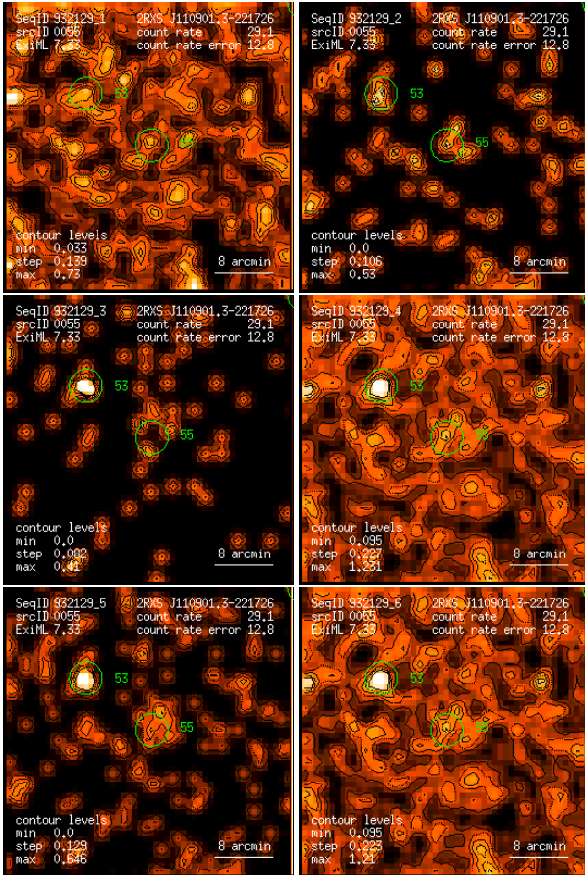
Figure 55: RASS 932129: detection 0055: band rate images, Gaussian filter: (1) PSPC channels 11 – 41, (2) 52 – 90, (3) 91 – 201, (4) 11 – 235, (5) 52 – 201, (6) 11 – 201. Broad band rates in counts/ks. Band rate contour levels in counts/ks/arcmin 2 .
