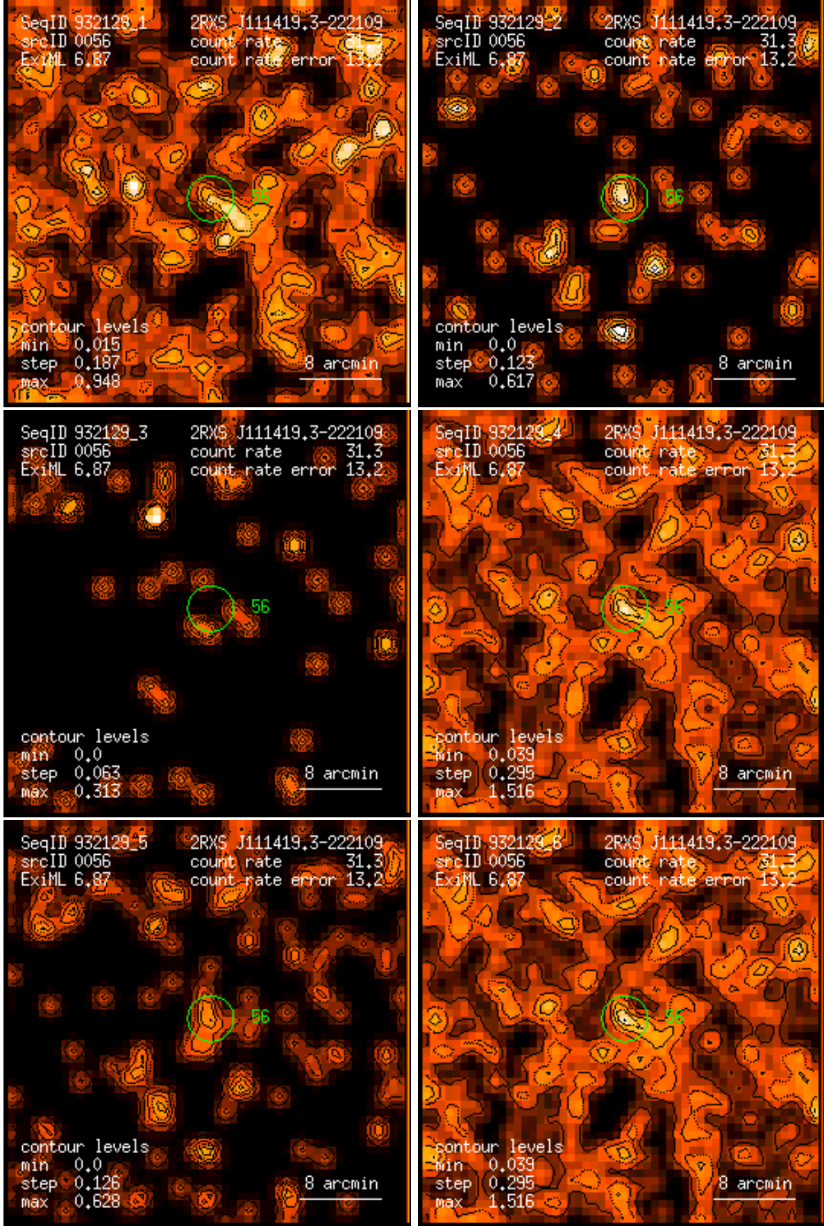
Figure 56: RASS 932129: detection 0056: band rate images, Gaussian filter: (1) PSPC channels 11 – 41, (2) 52 – 90, (3) 91 – 201, (4) 11 – 235, (5) 52 – 201, (6) 11 – 201. Broad band rates in counts/ks. Band rate contour levels in counts/ks/arcmin 2 .
