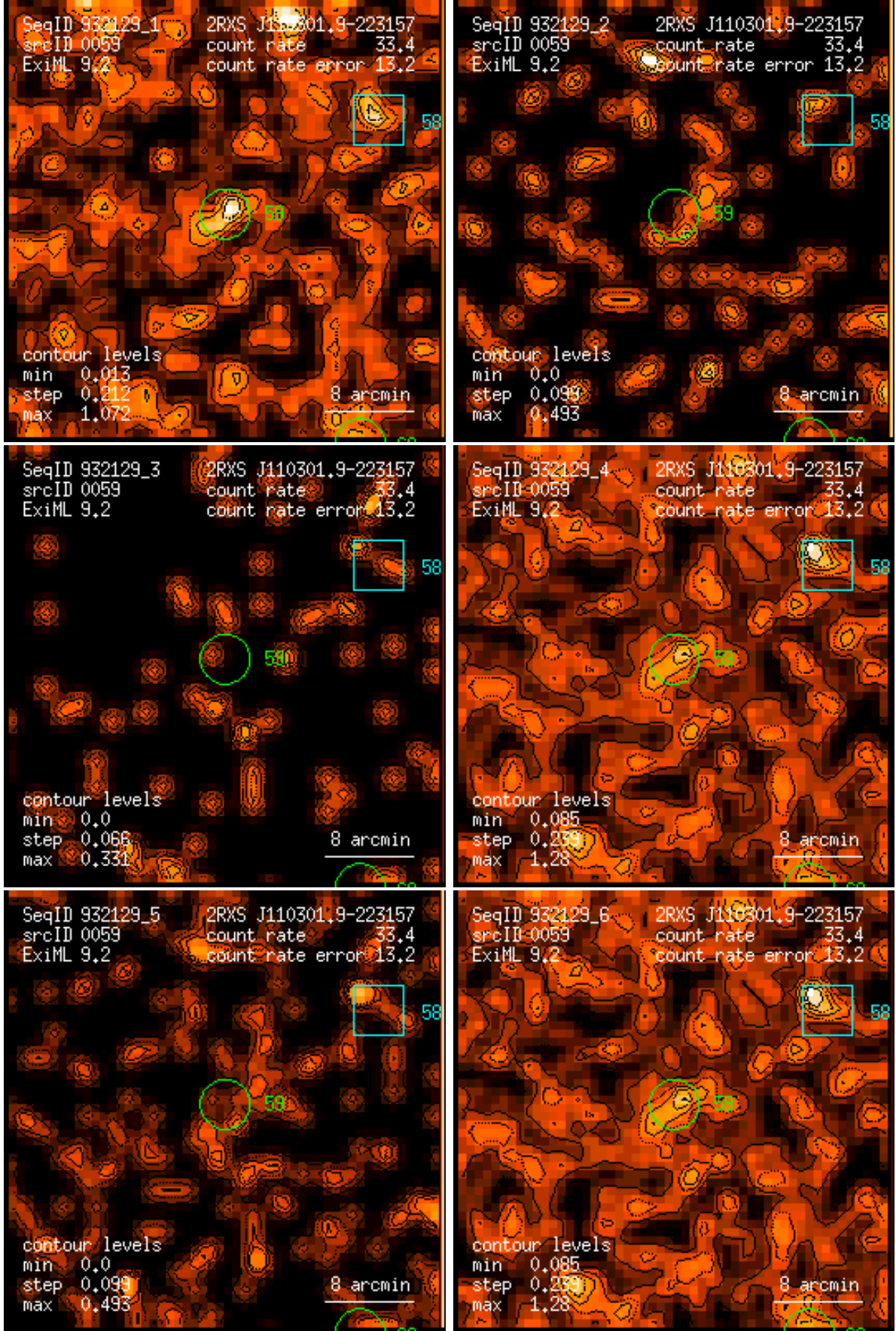
Figure 59: RASS 932129: detection 0059: band rate images, Gaussian filter: (1) PSPC channels 11 – 41, (2) 52 – 90, (3) 91 – 201, (4) 11 – 235, (5) 52 – 201, (6) 11 – 201. Broad band rates in counts/ks. Band rate contour levels in counts/ks/arcmin 2 .
